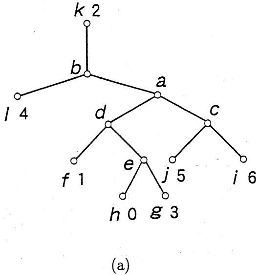
Figure 3: (a) A rooted el-tree (T_b, k) (b) The partial-ordering \leq_{\sigma(k)} = \leq_2
