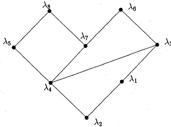
Figure 4: The MPR-poset (\mathbf{Rmp}(T), \leq_2)
