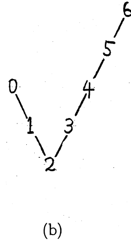
Figure 3: (a) A rooted el-tree (T_b, k) (b) The partial-ordering \leq_{\sigma(k)} = \leq_2
