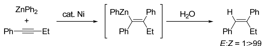
Scheme 4. Nickel-catalyzed arylzincation of alkynes.
