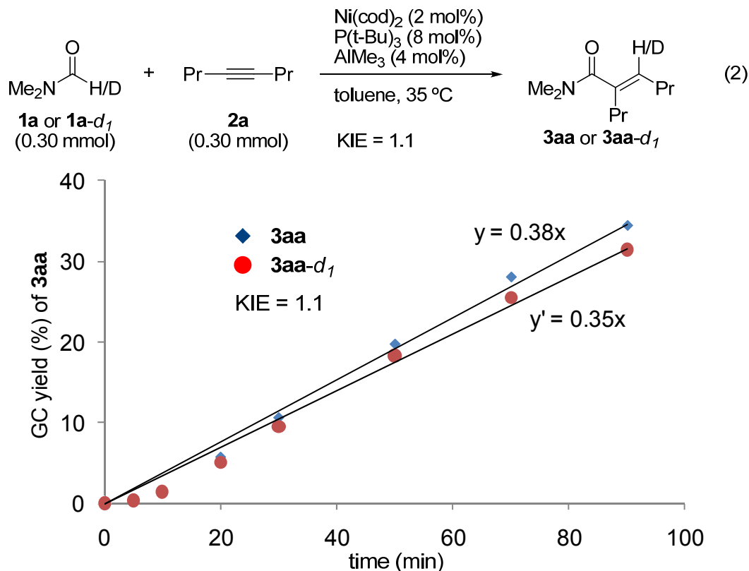
Figure 1. Estimation of KIE for hydrocarbamylation of alkynes
