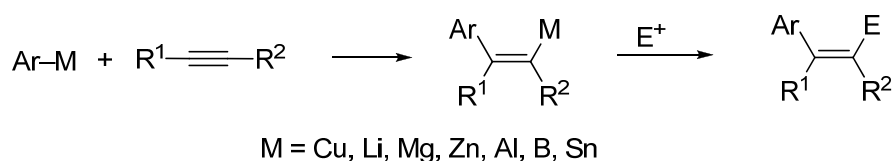
Scheme 2. Hydroarylation of alkynes through carbometalation followed by reactions with electrophiles.
