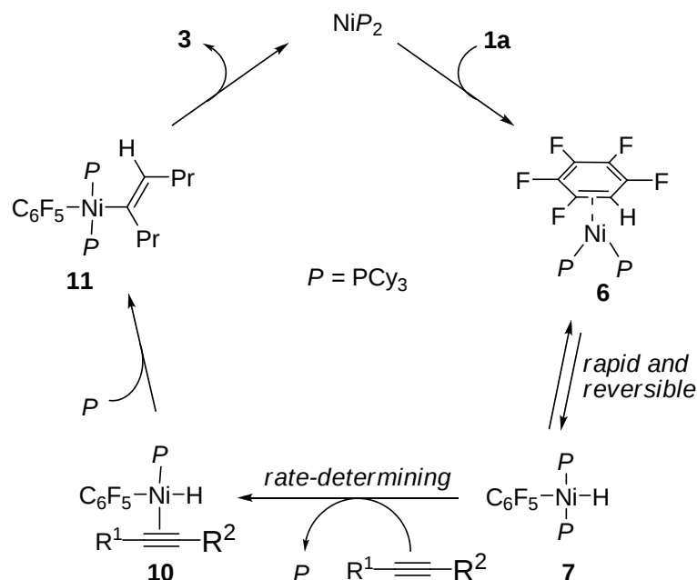
Scheme 2. Plausible mechanism for hydrofluoroarylation across alkynes.
