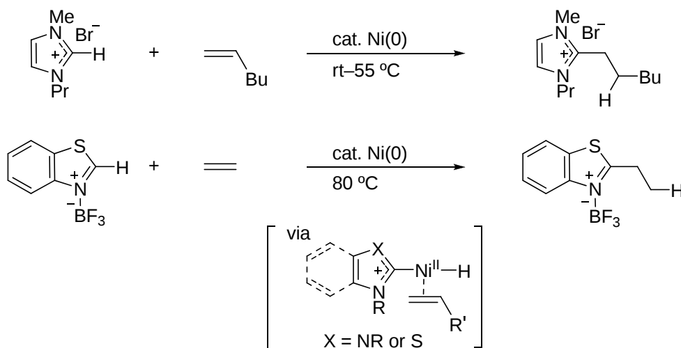
Scheme 14. Nickel-catalyzed olefin insertion into C(2)–H bonds in azolium salts.
