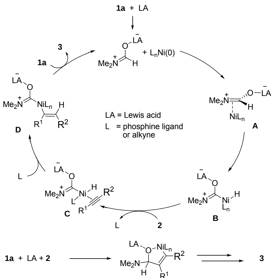
Scheme 2. Plausible reaction mechanism for the nickel/LA-catalyzed hydrocarbamylation of alkynes.
