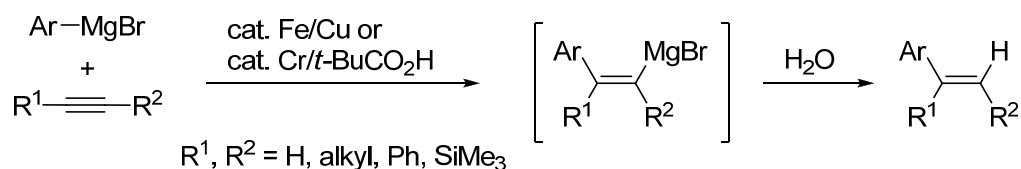
Scheme 3. Arylmagnesiation of alkynes catalyzed by iron/copper or chromium/pivalic acid.
