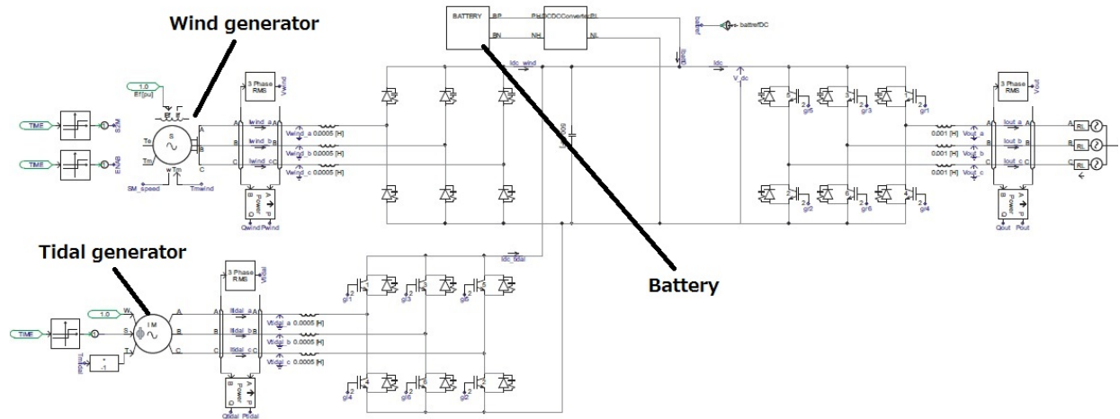
Fig. 5. HOTT with Battery System circuit.
