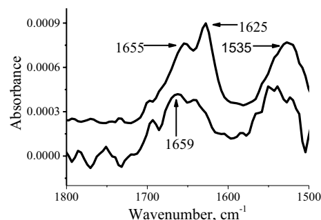
Fig. 3 pMAIRS results of the LB monolayer of the ^{13}\text{C} labeled \alpha -syn(61–95) at position 93G prepared at 10 mN/m on silicon slide. The top curve is the IP spectrum and the bottom one is OP spectrum
