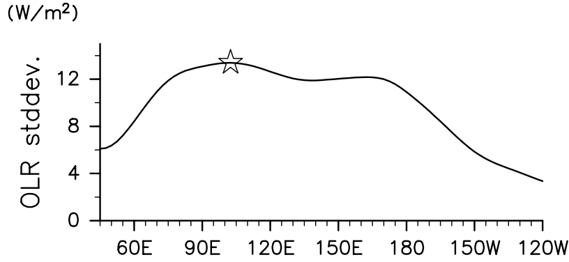
Fig. 4.3 Standard deviation at each longitude of the band-pass-filtered OLR data averaged over 5°N–15°S. The open star indicates the location of maximum standard deviation.
