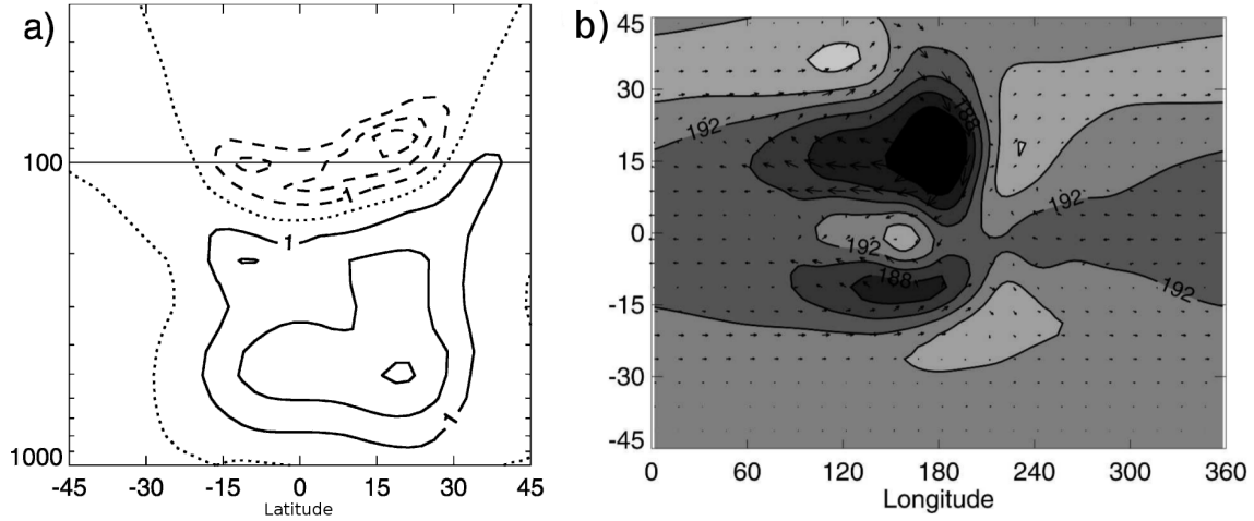
Fig. 1.5 (a) Zonal mean temperature response of the model with Gaussian heating centered at 15^\circ\text{N} . Contour interval is 1 K and solid contours indicate positive values and dashed contours negative values; dotted is the zero contour. (b) Temperature and wind vectors at 100 hPa from the model with heating centered at 15^\circ\text{N} . Contour interval is 2 K; darker shading indicates colder temperatures. From Norton [2006].
