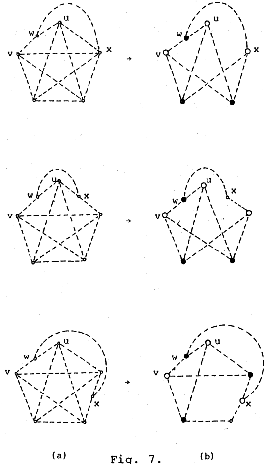
A subgraph of a graph G homeomorphic to K_{3,3} .
