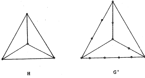
ig. 3. A graph G' homeomorphic to a graph H .
