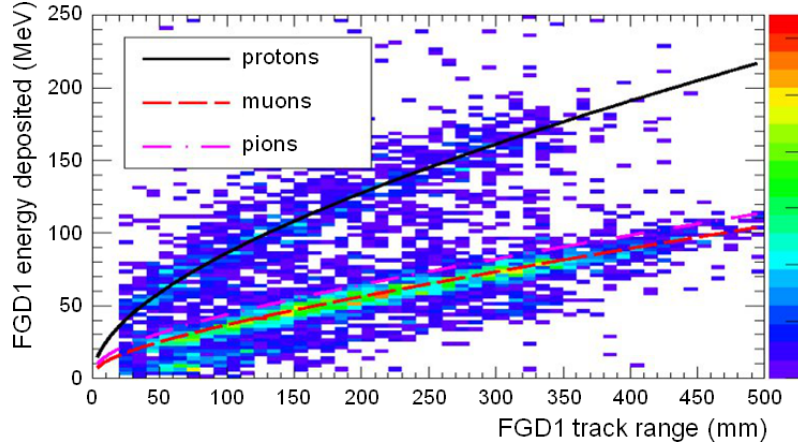
Figure 3.11: Deposited energy vs. stopping range for FGD1. The scatter-plot shows stopping particles in neutrino beam data, while the curves show the MC expectations for protons, muons, and pions [56].
