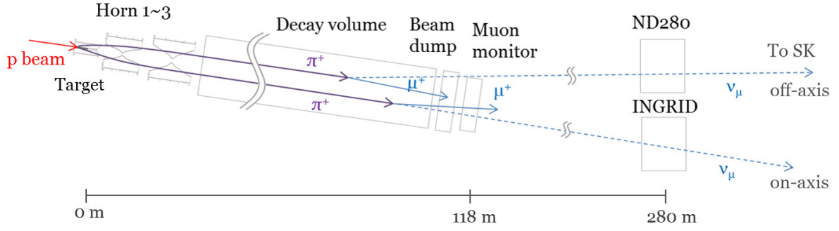
Figure 2.3: Neutrino beam line and the near detectors.
