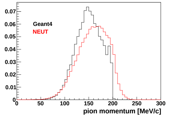
Figure A.15: Predicted momentum distribution of pions from inelastic scattering event, for Geant4 (black) and NEUT (red), for p_\pi = 201.6 MeV/c. The histograms are normalized by area.
