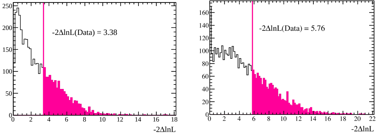
Figure 11.26: Distribution of -2\Delta\ln\mathcal{L}' at \delta_{\text{CP}} = \pi/2 , for 4000 toy MC experiments. The left (right) plot shows the distribution for the fit assuming normal (inverted) hierarchy. The pink line corresponds to the -2\Delta\ln\mathcal{L}' value obtained for data. The true values in MC is set to \sin^2 2\theta_{13} = 0.1 , \sin^2 \theta_{23} = 0.5 , \Delta m_{32}^2 = 2.4 \times 10^{-3} \text{ eV}^2 and \delta_{\text{CP}} = -\pi/2 .
