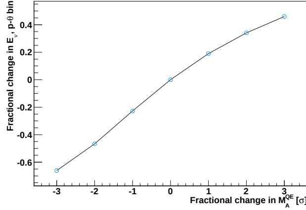
Figure 11.4: An example of a response function for p = 400\text{-}500 MeV/ c^2 , \theta = 60\text{-}70 degrees, E_\nu = 0.8\text{-}1.2 GeV.
