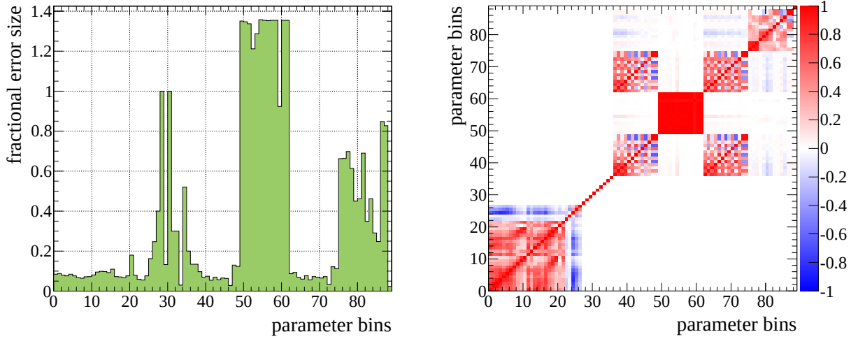
Figure 11.3: Size (left) and correlation matrix (right) of all the systematic uncertainties. The definition of the binning is shown in Table 11.3: 0-21=Beam parameters, 22-35=Cross section parameters, 36-87=SK efficiency+FSI+PN, 88=SK p-scape error. The definition of the beam parameter bins are same as the bins defined in Table 11.4, and the definition of the SK efficiency + FSI + PN parameters bins are same as in Fig. 10.6.
