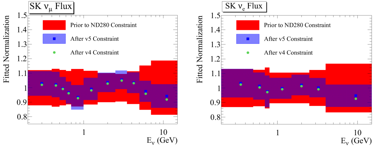
Figure 9.9: SK \nu_\mu (left) and \nu_e (right) flux parameters, before and after the fit. The red and blue bands represent the uncertainty of the parameters before and after the fit.
