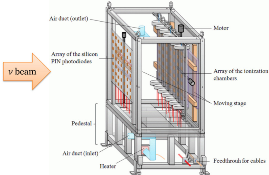
Figure 2.9: Schematic view of MUMON. Neutrino beam comes from the left side of the figure.
