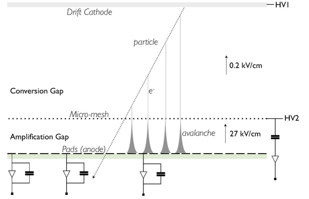
Figure 2.14: TPC micromegas readout.
