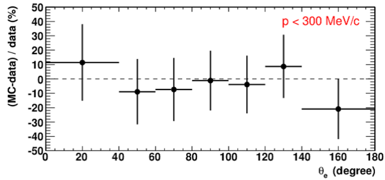
Figure D.2: Example of the data/MC relative difference in NC1 \pi^0 hybrid- \pi^0 control sample for the \theta_e bins, at p_e < 300 MeV/c.
