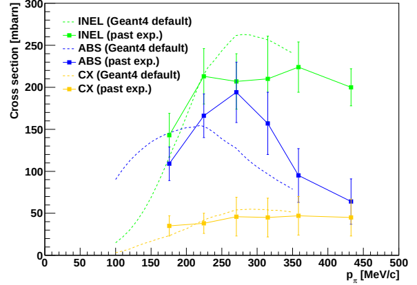
Figure 5.8: Comparison of inelastic inclusive cross sections between the past experiment [70] and Geant4 default. The cross sections are plotted as a function of pion momentum.
