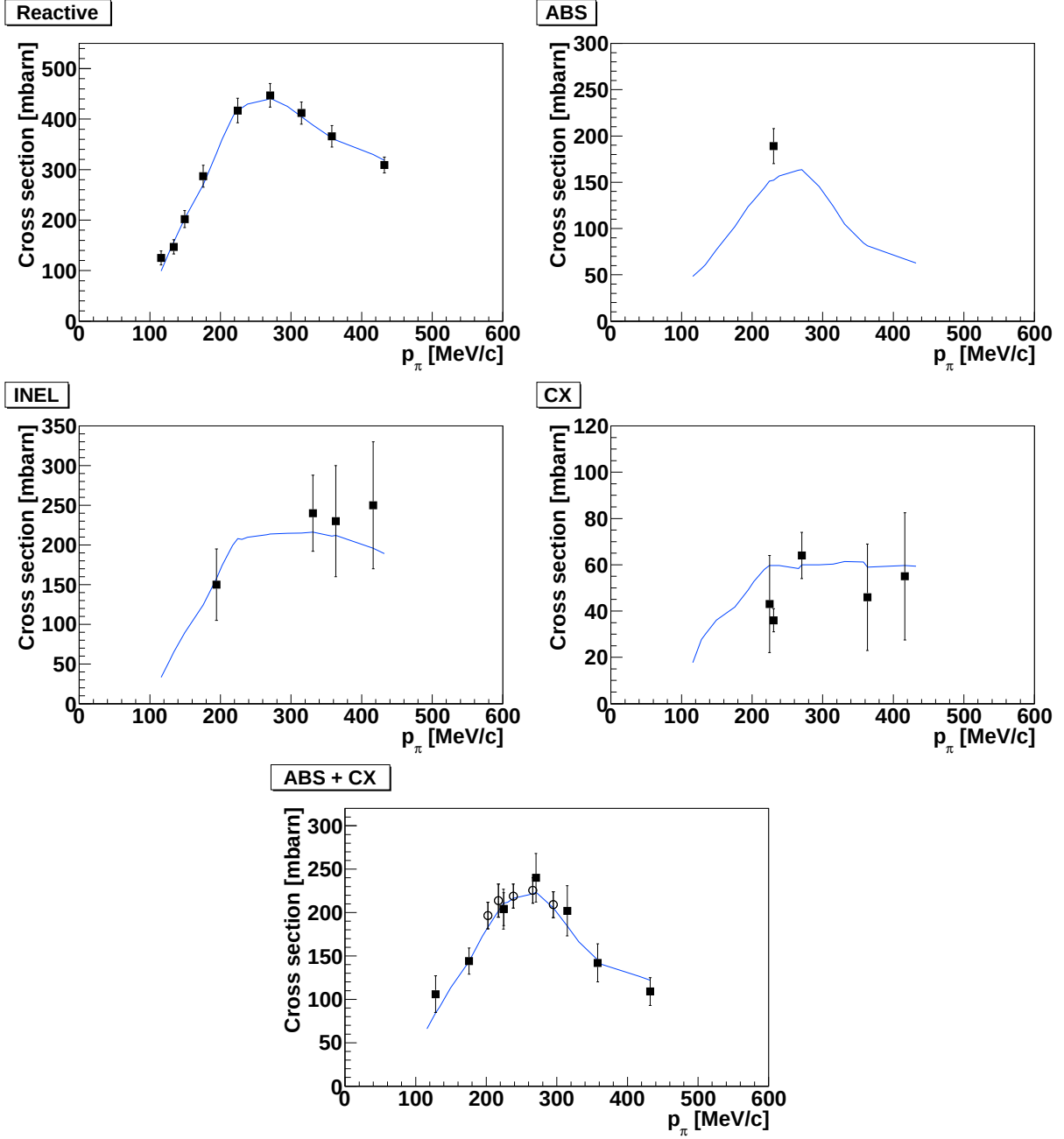
Figure 6.5: \pi^+-^{12}\text{C} cross section for five different interaction channels, compared between NEUT nominal prediction (blue curves) and data points from past experiments. The white circle points in ABS + CX sample are the data points from our measurements.
