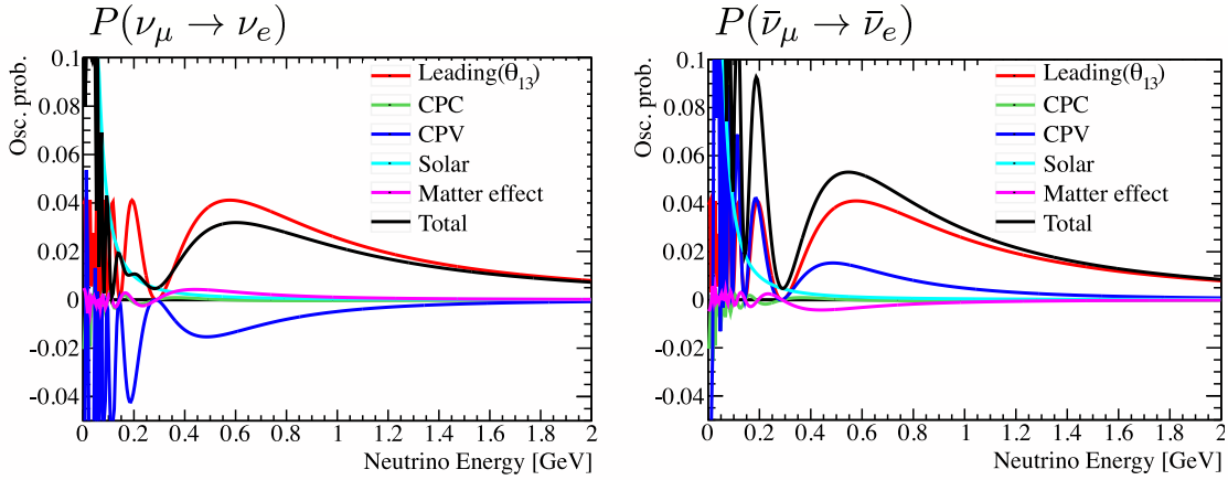
Figure 1.2: The \nu_\mu \rightarrow \nu_e and \bar{\nu}_\mu \rightarrow \bar{\nu}_e oscillation probability as a function of neutrino energy, with \sin^2 2\theta_{13} = 0.098 , \delta_{CP} = \pi/2 , \sin^2 2\theta_{23} = 0.97 , |\Delta m_{32}^2| = 2.35 \times 10^{-3} \text{eV}^2 , normal hierarchy and baseline of 295 km.
