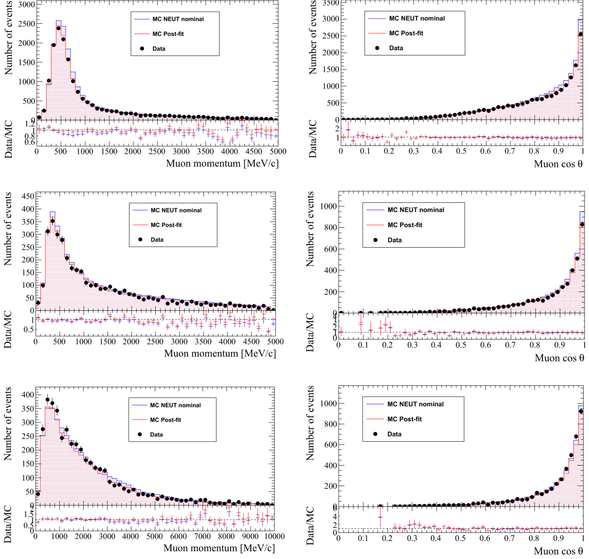
Figure 9.8: Muon momentum and \cos \theta distribution for data compared with MC, for CC0 \pi sample (top), CC1 \pi sample (middle) and CC-Other sample (bottom). The blue and red histograms shows the MC distributions before and after data constraint, respectively.
