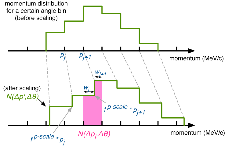
Figure 11.5: An illustration of the implementation of the SK momentum scale error.
