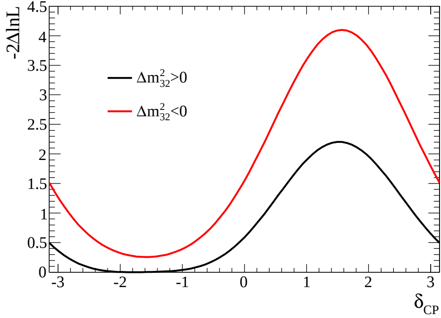
Figure 11.27: Negative log delta likelihood as a function of \delta_{\text{CP}} , averaged over 4000 toy MC experiments, for 6.570 \times 10^{20} POT case. Black (red) curve shows normal (inverted) hierarchy case. Likelihoods are marginalized over \sin^2 \theta_{23} , \Delta m^2_{32} and \sin^2 2\theta_{13} .
