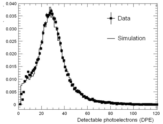
Figure 3.10: Charge distribution after correction, compared with simulation [56].
