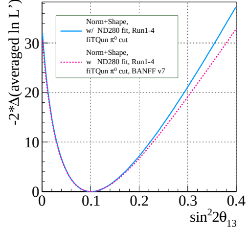
Figure 11.12: Negative averaged log likelihood as a function of \sin^2 2\theta_{13} with old 2012 systematic errors (pink) and with new 2013 systematic errors (blue), for Run1-4 POT case.
