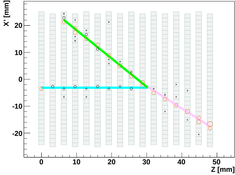
Figure 5.1: Example of ABS candidate event in data ( p_\pi = 250 \text{ MeV}/c ). The red circles correspond to the large hits ( > 20 p.e.), and the crosses correspond to the hits identified as crosstalk hits.
