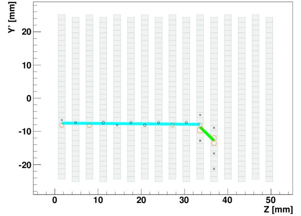
Figure 5.3: Example of CX candidate event in data ( p_\pi = 250 \text{ MeV}/c ). The blue track is assumed to be the incident pion track, and the green track is assumed to be a proton track from CX interaction.
