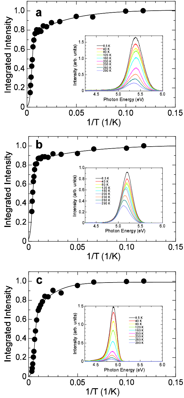
Figure 4.19: Arrhenius plot of integrated PL of Al 0.79 Ga 0.21 N/AlN QWs with L_z of (a) 2.6 nm, (b) 5.2 nm and (c) 10.4 nm. Inset figure shows their corresponding PL spectra.
