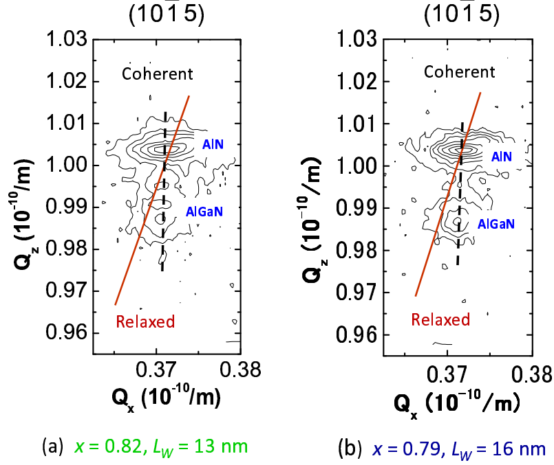
Figure 4.5: Reciprocal space mapping (RSM) of L_w \sim 13 and \sim 16 nm \text{Al}_x\text{Ga}_{1-x}\text{N}/\text{AlN} QWs.
