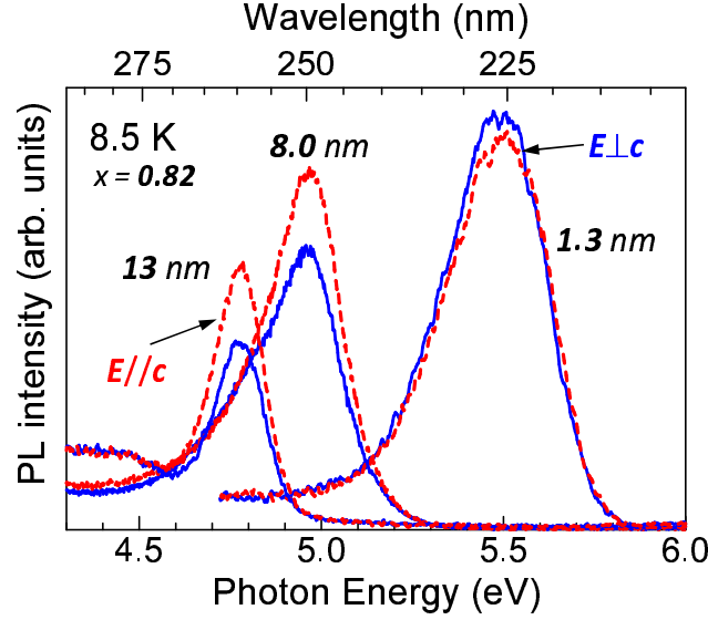
Figure 5.7: Polarization PL spectra of c-oriented \text{Al}_{0.82}\text{Ga}_{0.18}\text{N}/\text{AlN} MQWs with different well widths ( L_w ) of 1.3, 8.0, and 13 nm. The polarization changed from ( \mathbf{E} \parallel c ) to ( \mathbf{E} \perp c ) as the well width ( L_w ) is decreased.
