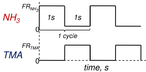
Figure 2.4: Alternating supply sequence of TMA and NH_3 in MEE. This method was first applied in GaAs and AlAs-GaAs system then eventually adapted for AlN growth.
