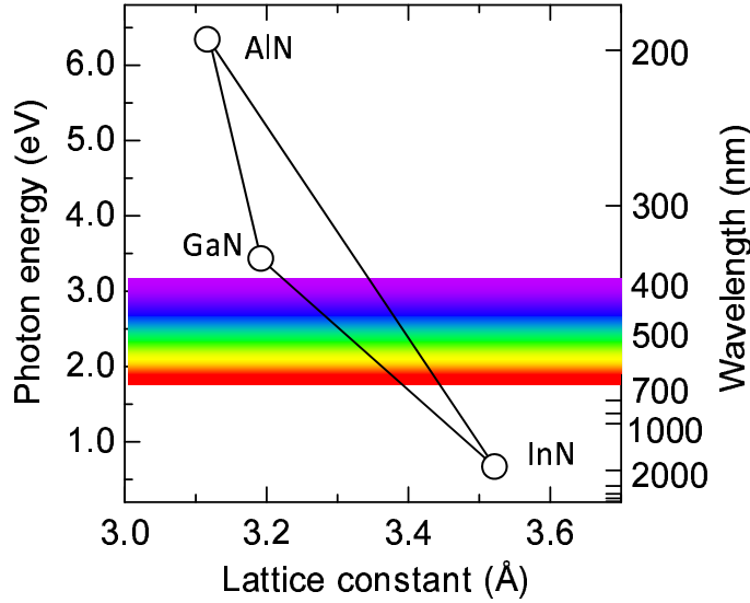
Figure 1.1: The lattice constants ( a_0 ) of binary III-V semiconductors compounds plotted against their corresponding bandgap energy and wavelength at room temperature.
