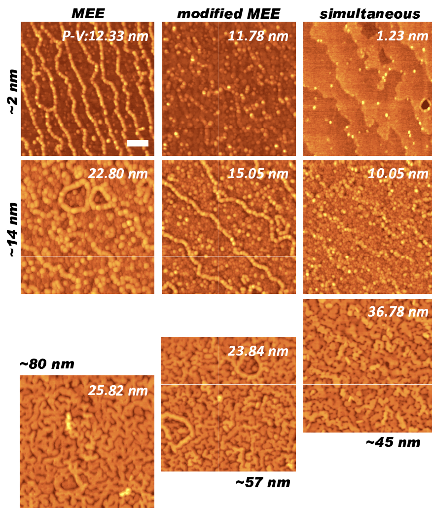
Figure 2.9: AFM images of AlN by MEE, modified MEE and simultaneous supply showing the evolution of initial nucleation. Thicknesses of ~2 and ~14 nm are nominal. The scale bar represents 20 nm.
