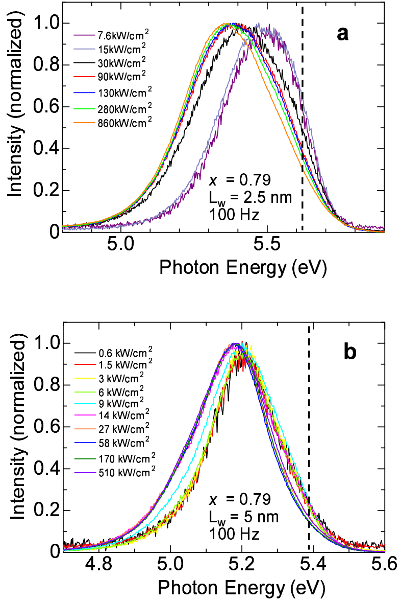
Figure 4.24: PL spectra of Al 0.79 Ga 0.21 N/AlN QWs with well width of (a) 2.5 nm and (b) 5 nm well width. The position peaks moves closer to the calculated transition energy with decreasing power density.
