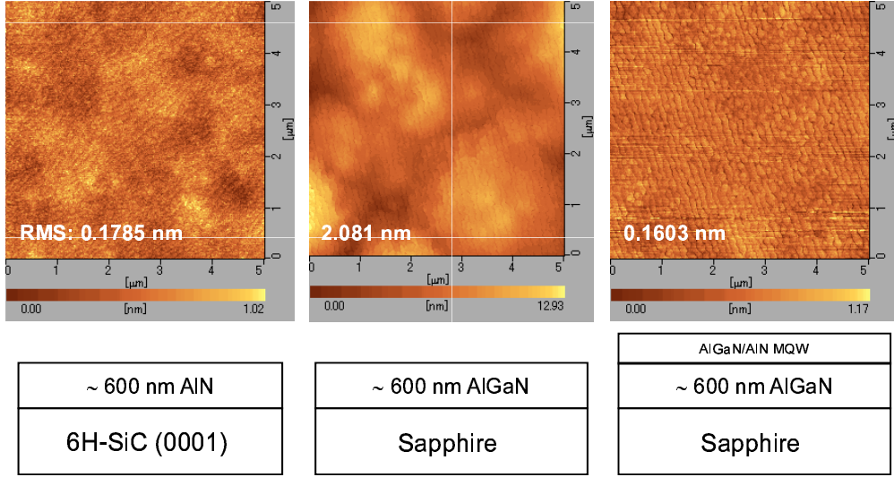
Figure 3.19: The different material systems used to fabricate thick AlN and AlGaIn, and AlGaIn/AlN MQWs.
