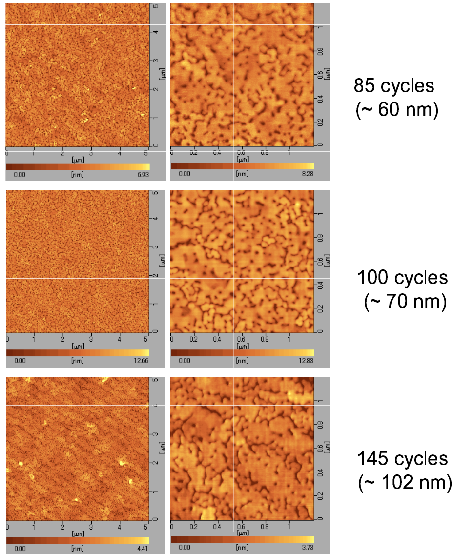
Figure 3.10: AFM images of structural evolution of AlN fabricated by Modified MEE. AlN epilayers were grown for 85 cycle, 100 cycles and 145 cycles. Left figure scan area: 5 \times 5 \mu\text{m} . Right: 1.2 \times 1.2 \mu\text{m}
