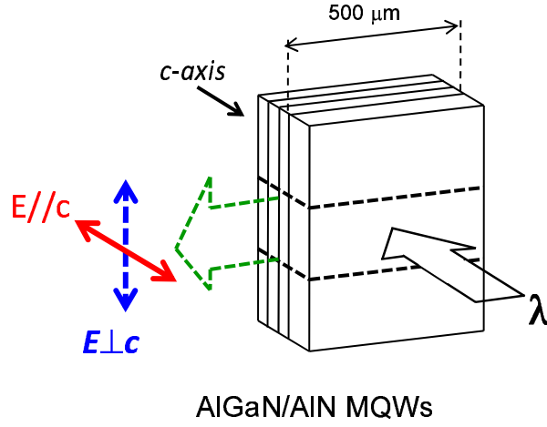
Figure 5.4: Schematic AlGaIn/AlN MQWs samples cleaved along the m-plane with respect to AlN used for optical polarization experiments. Using this this set-up, the \mathbf{E} \perp c and \mathbf{E} \parallel c components are clearly resolved.
