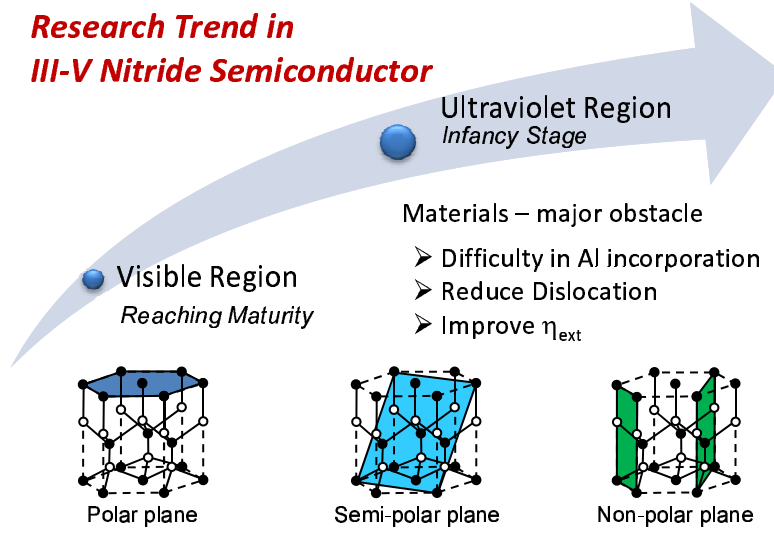
Figure 1.2: Current research trend in the study of III-V nitrides. While the visible region has improved by leaps and bounds in terms of epitaxy and efficiency, the ultraviolet region has just started attract interests. As shown, the foremost concern to obtain high-efficiency UV devices is to improve the material.
