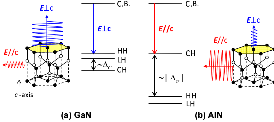
Figure 5.2: The difference in crystal-field splitting energy of (a) GaN and (b) leads to the unique optical polarization properties in AlGaIn. While an intense emission from the c-plane is expected from GaN, weaker surface emission is expected for AlN due to their differences in crystal-field energy ( \Delta_{cr} ).
