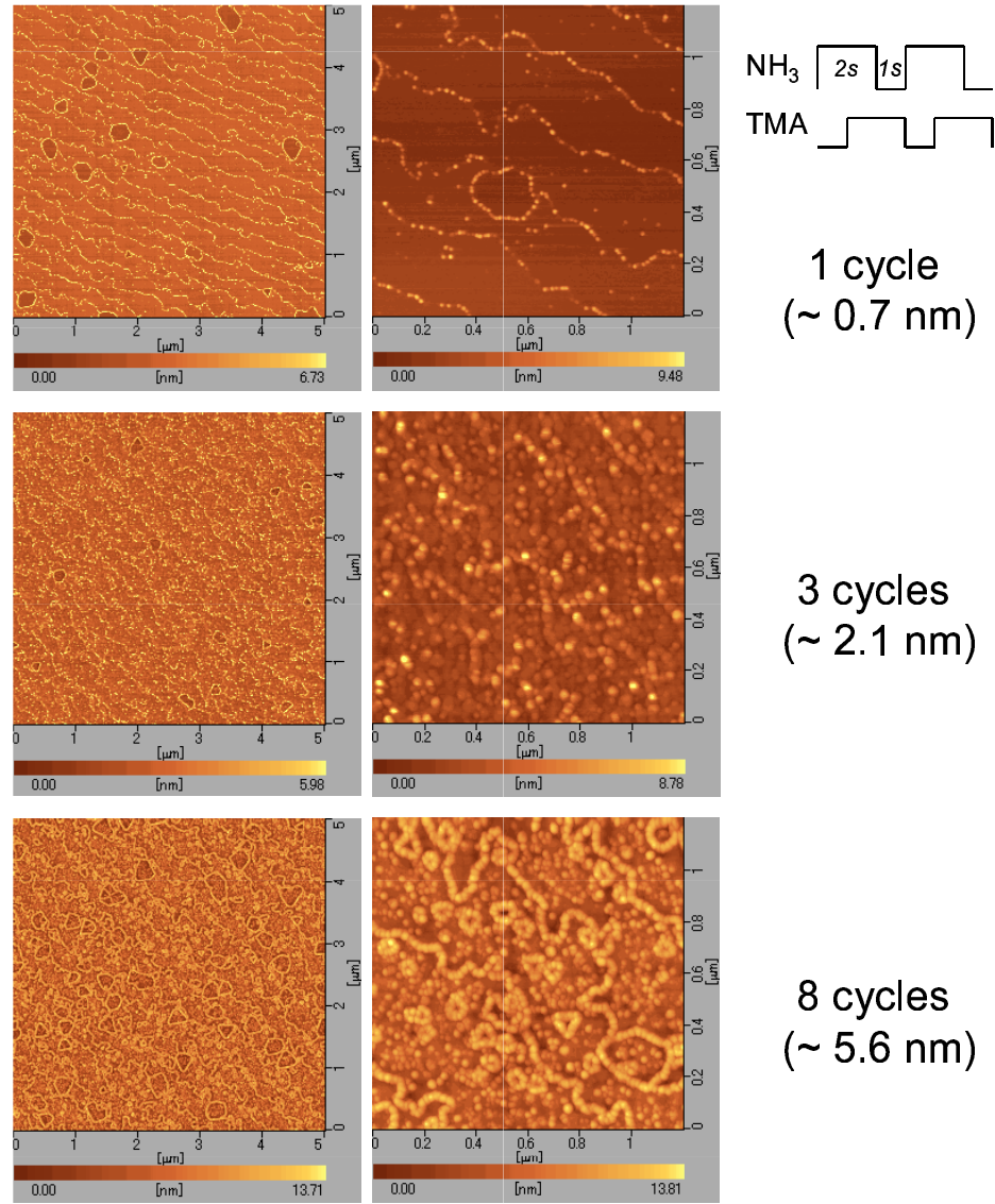
Figure 3.8: AFM images of structural evolution of AlN fabricated by Modified MEE. AlN epilayers were grown for 1 cycle, 3 cycles and 8 cycles. Left figure scan area: 5 x 5 μm. Right: 1.2 x 1.2 μm
