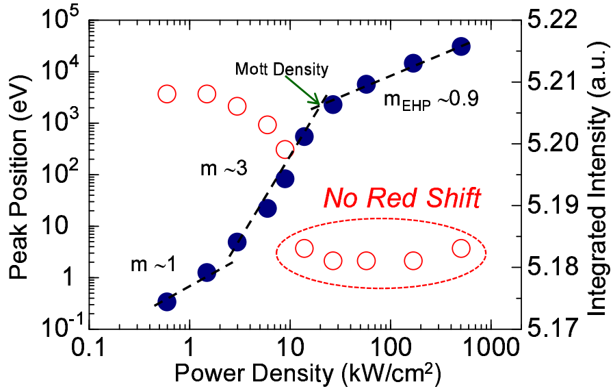
Figure 4.26: The plot of the excitation power density with peak position and PL intensity for the sample with the highest \eta (Al 0.79 Ga 0.21 N/AlN QWs, L_w = 2.5 nm). No red-shift was observed with increasing excitation density - an anomalous behavior worthy of further analysis.
