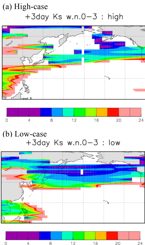
Fig. 4 Stationary wave number Ks for the observed basic wind fields at 850 hPa at 3 days after the initial time of the forecast. The basic wind field is composed of zonal wavenumber 0-3 components. (a) High-case, (b) Low-case.
