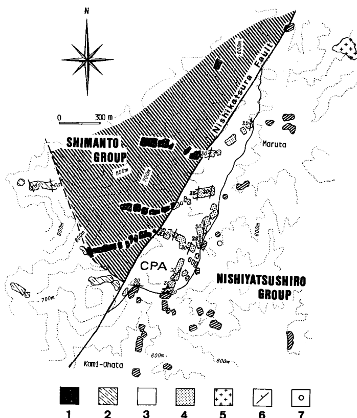
Fig. 15. Topographic map with location of outcrops in Maruta, see Fig. 6 for map location. Note that CPA directly abut to the underlying Nishiyatsushiro Group. 1. black shale of "Shimanto Group", 2. alternations of sandstone and mudstone (Kawaguchi Formation, Nishiyatsushiro group), 3. altered pyroclastics (Onuma Formation, Nishiyatsushiro group), 4. Conglomerate-sandstone association (CPA), 5. intrusive rocks (porphyrite), 6. dip and strike, 7. floating block.
