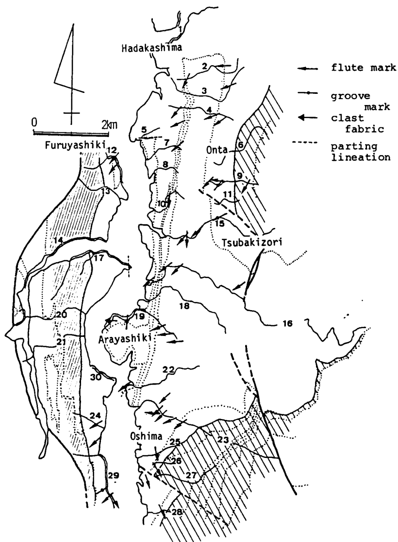
Fig. 23. Paleocurrent directions of SDA, GSA and SIA in Minobu area, showing fairly constant west-southwest transposing, and concordant with that of the three facies associations.
