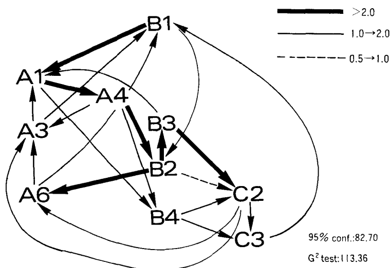
Fig. 18. Transitional pattern of sedimentary facies of SCA, showing fining-upward sequence.
