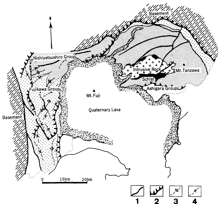
Fig. 3. Generalized geological and structural map of the Southern Fossa Magna Region, showing half-dome structure facing north around Tanzawa mountain, of the Miocene System. 1. Fault, 2. Thrust, 3. Anticline, 4. Syncline.
