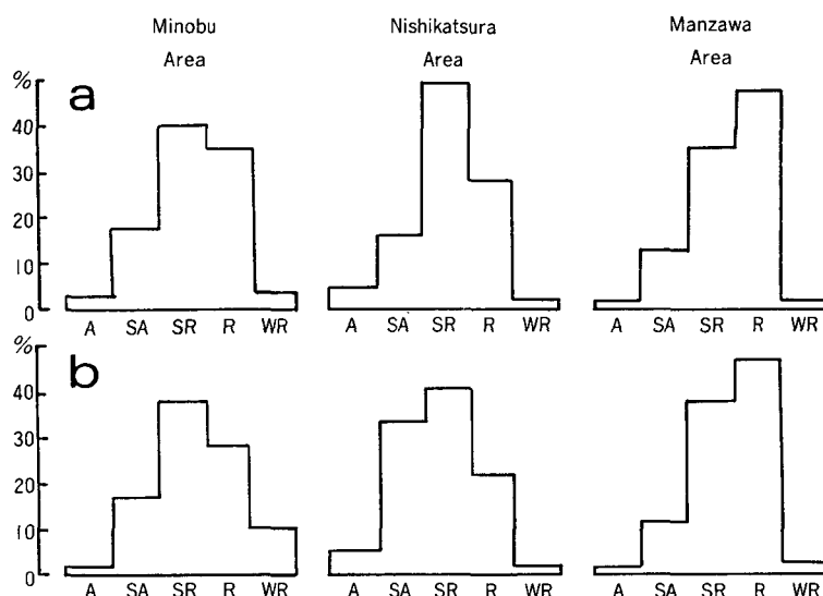
Fig. 30. Roundness of sandstone and shale clasts. a: sandstone, b: black shale, A: angular, SA: subangular, SR: subrounded, R: rounded, WR: well-rounded.
