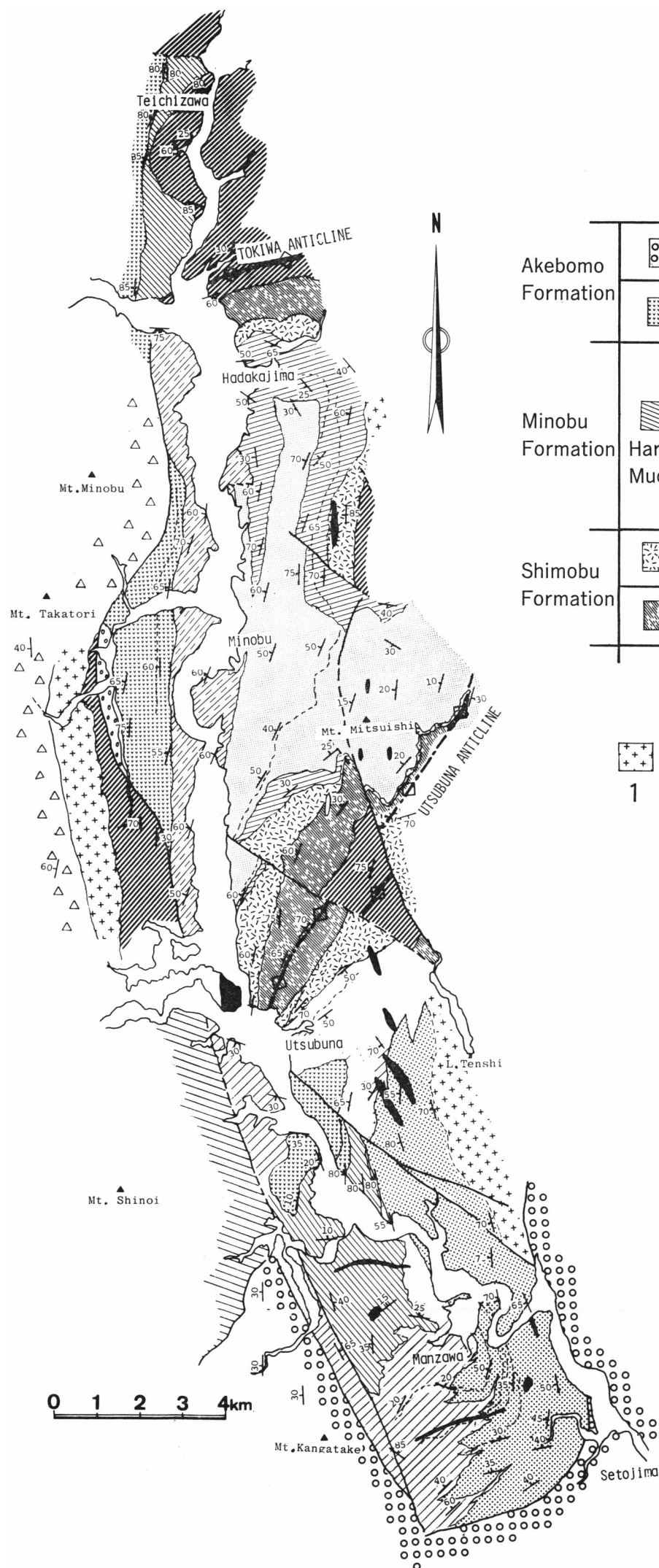
Fig. 5. Geological map of Fujikawa domain. The boundaries of Akebono and Minobu, and Minobu and Manzawa areas are drawn on the axes of the Tokiwa and Utsubuna Anti clines. 1. Intrusive rocks, 2. dyke rocks, 3. fault, 4. dip and strike.
