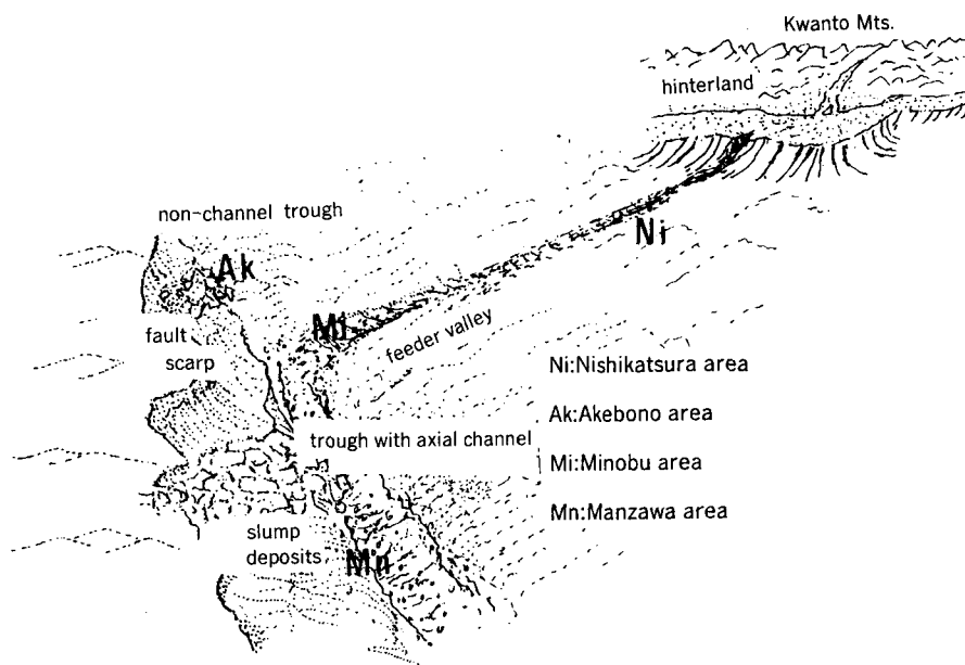
Fig. 35. Reconstructional models of sedimentary setting of the western half of the Southern Fossa Magna Region.
