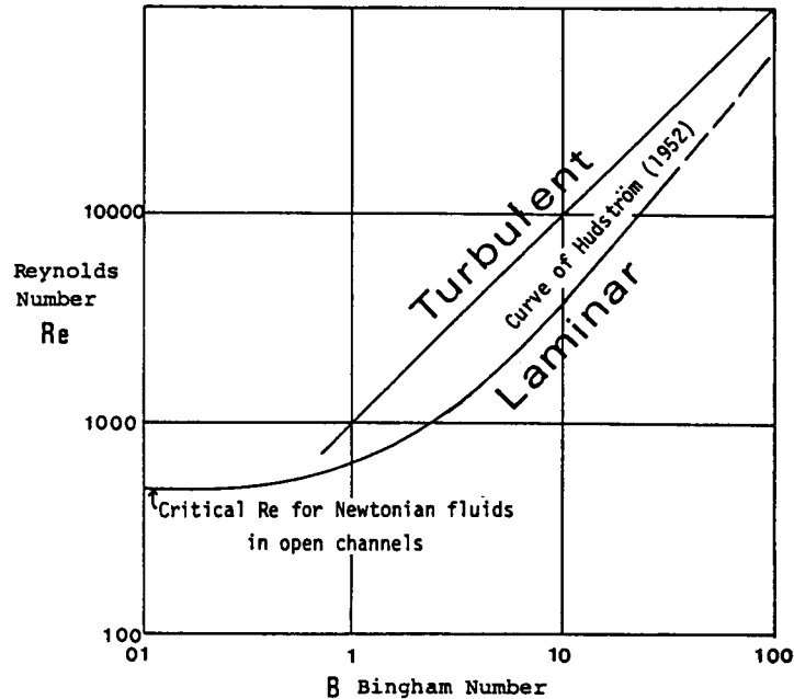
Fig. 33. Transitional condition of Bingham material from laminar fashion to turbulent one (after Hiscot & Middleton, 1979).
