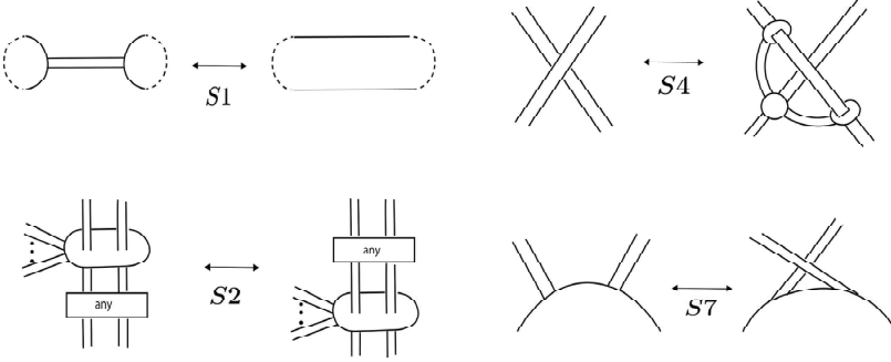
Figure 8: Example of moves of ribbon presentations
