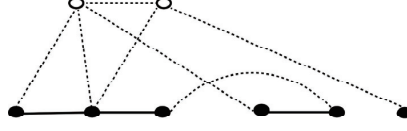
Figure 1: Example of an admissible plain graph
