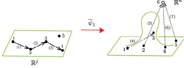
Figure 14: Example of the direction map
