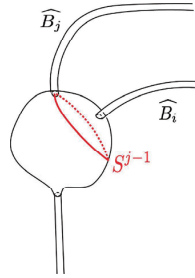
Figure 11: The additional S^{j-1} family
