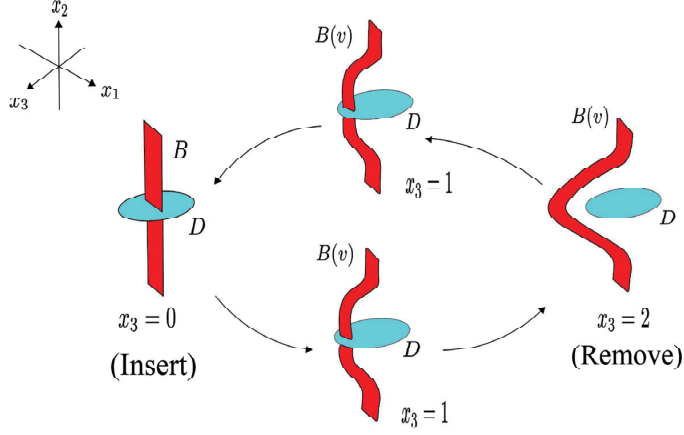
Figure 10: Perturbation of a crossing ( n - j = 3 )
