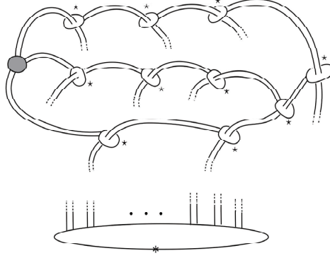
Figure 9: The ribbon presentation P(\Theta(4, 3, 2))
