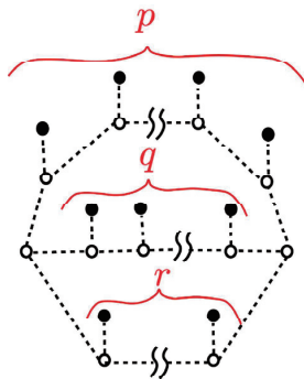
Figure 4: The hairy graph \Theta(p, q, r)
