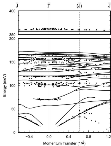
FIG. 4. Surface-phonon dispersions of C(001)(2 \times 1)-H along the \Gamma J and \Gamma J' high-symmetry lines. The solid curves represent calculated bands. The modes with small contribution from the surface are not drawn, and thus, some branches are disconnected in the SBZ. The dots show the mode energies, as determined from the EELS data. Since both 1 \times 2 and 2 \times 1 domains coexist at the sample surface, the experimental data are superimposed in both directions. The dashed vertical line indicates the ( J ) point of the 1 \times 2 SBZ.
