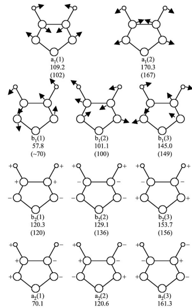
FIG. 3. Schematic displacement patterns of salient normal modes at the \Gamma point. They are classified according to the irreducible representations of the C_{2v} point group. The calculated energy of each mode, to which an observed loss peak is assigned, is shown with the respective measured energy in brackets (in units of meV). Only the a_1 , b_1 , and b_2 modes are observable in EELS.
