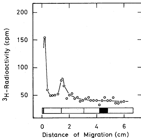
Fig. 5. SDS-polyacrylamide gel electrophoresis on 10% gel of fd labelled with ^3\text{H} -Histidine and dissociated in 0.1% SDS solution. The anode is taken to the right. The insert at the bottom represents a rough sketch of the staining. The bands indicate, from left to right, A-protein aggregate, A-protein monomer, presumably contaminated cell protein, and the major component of B-protein.
