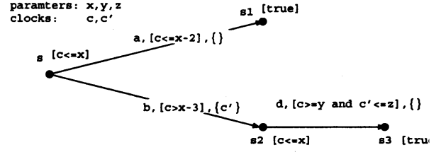
Fig. 1: Example of Parametric Timed Automata
