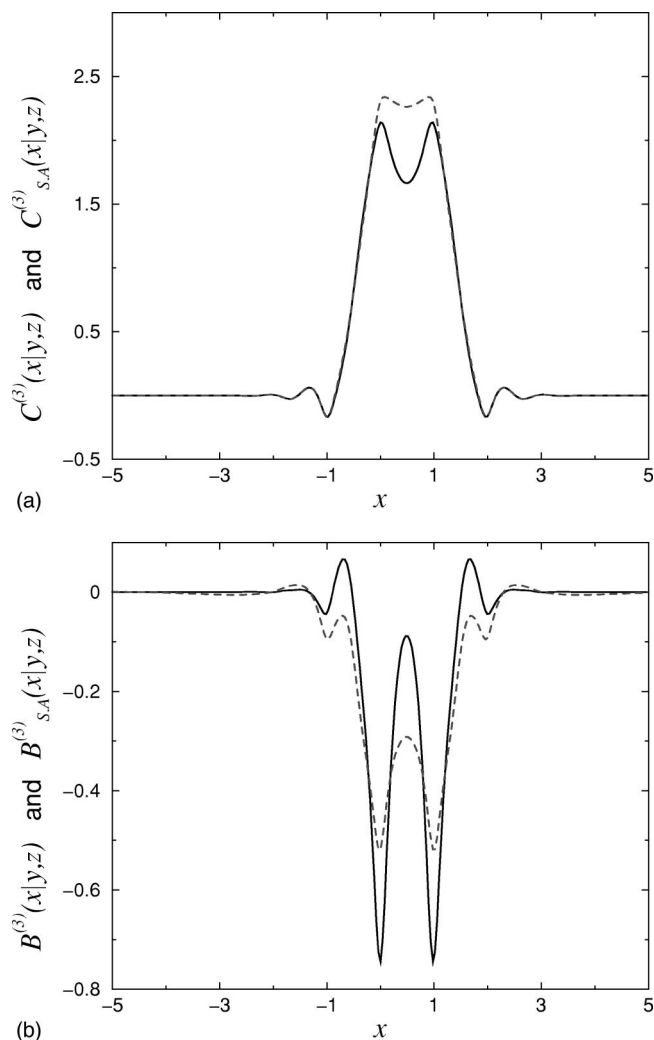
FIG. 3. (a) C^{(3)}(x|y,z) (a dashed curve) from the M=3 HNC theory and the superposition approximation C_{SA}^{(3)}(x|y,z) (a solid curve) for y/l=0.98 and z/l=0 . (b) B^{(3)}(x|y,z) (a dashed curve) from the M=3 HNC theory and the superposition approximation B_{SA}^{(3)}(x|y,z) (a solid curve) for y/l=0.98 and z/l=0 .
