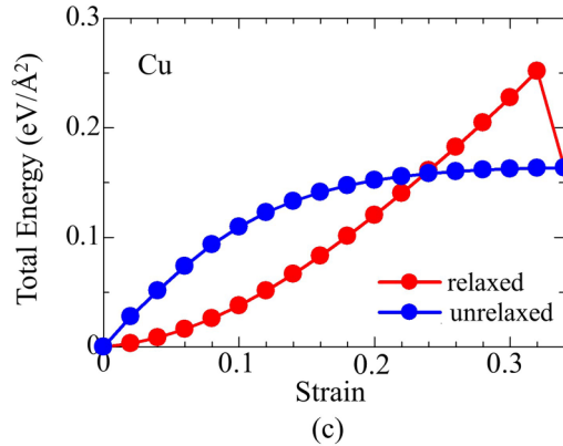
FIG. 1. Variation in the total energies of the (a) \beta -SiC, (b) Ge, and (c) Cu cells as a function of strain. The variation in the total energy was determined by relaxed-type and unrelaxed-type first-principles tensile tests. In the unrelaxed-type simulations, the separation planes move along the tensile direction with all of the atoms fixed. In the relaxed-type simulations, only the atoms located in the outermost two layers of the cell are fixed for tensile straining, while the other atoms can move freely. The total energy is found to continuously vary in the unrelaxed-type simulations. In the relaxed-type simulations, after the total energy continuously varies, it suddenly decreases in the final stage.
