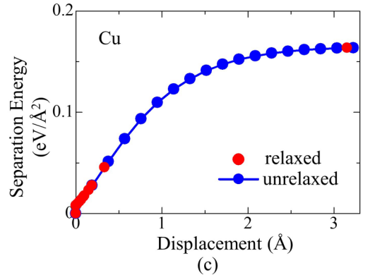
FIG. 2. Variation in the inelastic separation energy of the separation planes as a function of the displacement between them: (a) \beta -SiC, (b) Ge, and (c) Cu. The variation in the inelastic separation energy was determined by relaxed-type and the unrelaxed-type first-principles tensile tests. The inelastic separation energy continuously is found to vary in the unrelaxed-type simulations. In the relaxed-type simulations, the inelastic separation energy continuously varies until a certain displacement, and it then discontinuously jumps to its final value. The stress at the onset of the energy jump can be defined with the fracture stress. Although it appears that the number of data for the relaxed-type test is less than that for the unrelaxed-type test, some data for the relaxed-type test overlap, and the number of data for the relaxed-type test is the same as that for the unrelaxed-type test.
