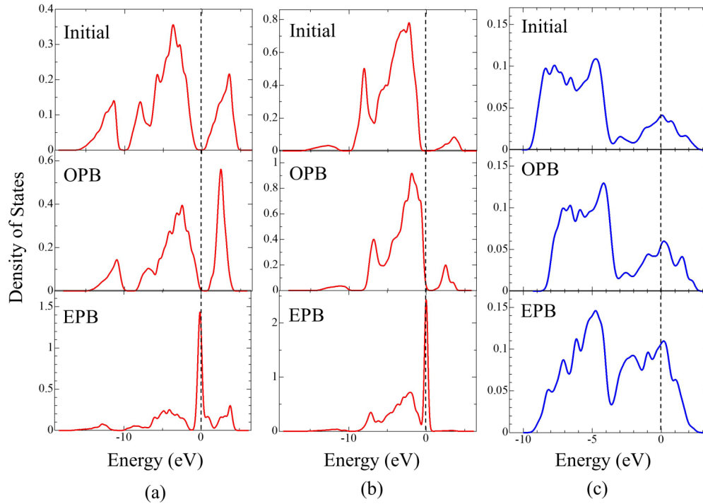
FIG. 4. Partial DOS before deformation (initial), at the OPB and at the EPB for \beta -SiC and Cu. (a) p orbitals of a Si atom, (b) p orbitals of a C atom, and (c) s orbitals of a Cu atom at the separation plane before deformation, at the OPB, and at the EPB. The partial DOS at the OPB is similar to that before deformation. The electrons are localized near the Fermi level at the EPB.
