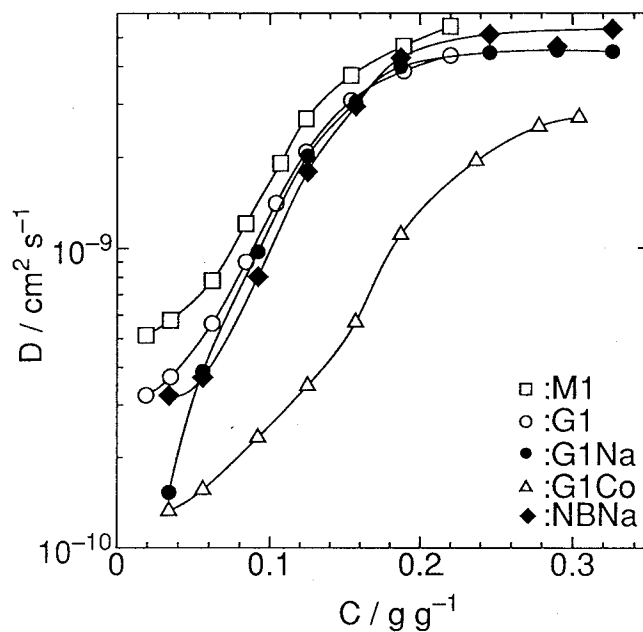
Figure 10. Concentration dependence of integral diffusion coefficient at 30°C. \square : M1, \circ : G1, \bullet : G1Na, \triangle : G1Co, \blacklozenge : NBNa.
