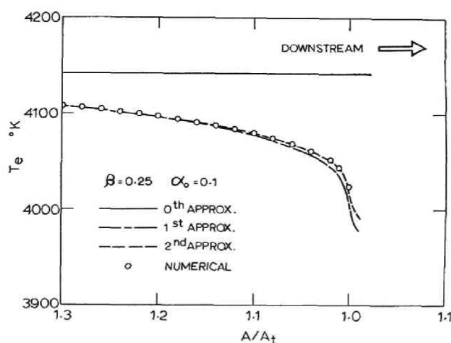
Fig. 7 Distribution of temperature T for an equilibrium flow along the nozzle axis.
