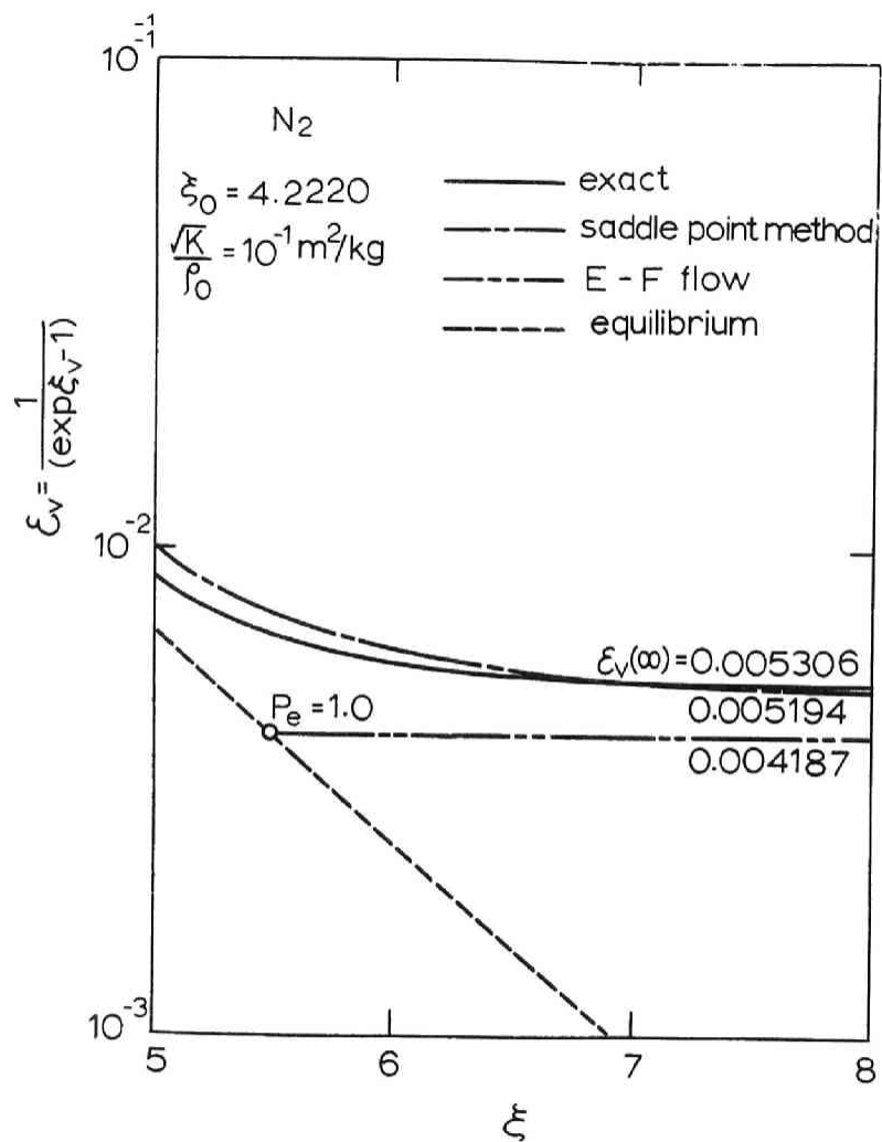
Fig. 11 Distributions of vibrational energy.
