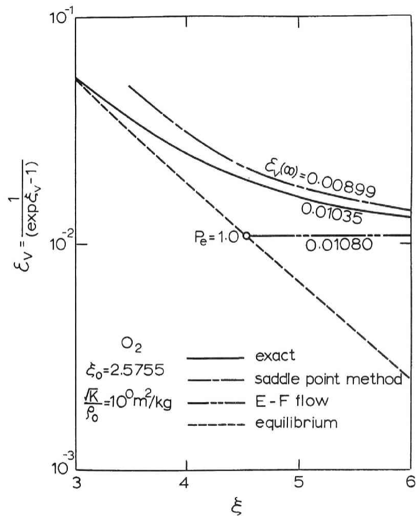
Fig. 11 Distributions of vibrational energy.
