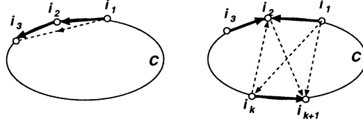
Figure 3: x_{i_1 i_2} and x_{i_2 i_3} (left) or x_{i_1 i_2} and x_{i_k i_{k+1}} (right) appear in \text{in}_{\prec}(f_C) .
