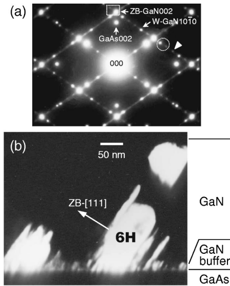
FIG. 1. (a) ED pattern and (b) TEM dark-field image of GaN grown on GaAs(001). The (110) cross section was observed. The arrowhead in (a) shows one of the diffraction spots from six-bilayer periodic structures. Also in (a), the circle indicates the size of the objective aperture, inside which are the diffraction spots used to generate the dark-field image of (b). The rectangle in (a) is used with Fig. 3.
