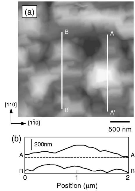
FIG. 5. Surface structures of GaN including the six-bilayer periodic structures: (a) AFM image and (b) height profiles measured along AA' and BB' in (a).
