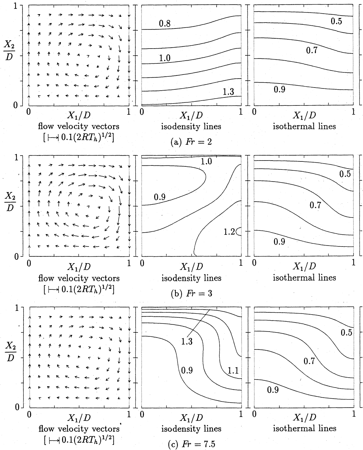
Fig. 4. Flow velocity vectors, isodensity lines, and isothermal lines for three Froude numbers, Fr = 2, 3 , and 7.5 , with L/D = 1 , Kn = 0.02 , and T_c/T_h = 0.4 . (a) Fr = 2 , (b) Fr = 3 , and (c) Fr = 7.5 . The arrows indicate the velocity at their starting points. The contours \rho/\rho_0 = 0.1n and T/T_h = 0.1n are shown. [The (X_1, X_2) space is divided into 48 \times 48 [in (a) and (b)] or 72 \times 72 [in (c)] nonuniform rectangular lattices finer near the upper and right boundaries. The (\xi_1, \xi_2) space, limited to |\xi_1| and |\xi_2| \leq 4(2RT_h)^{1/2} , is divided into 40 \times 80 [in (a)], 40 \times 60 [in (b)], or 40 \times 40 [in (c)] nonuniform rectangular lattices, finer near the lines \xi_1 = 0 and \xi_2 = 0 .]
