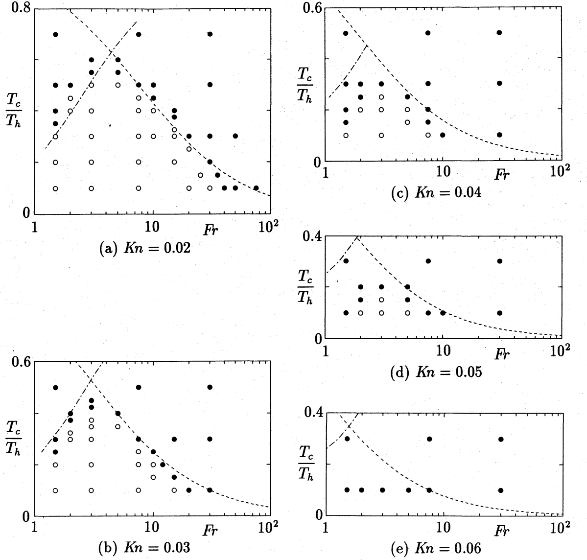
Fig. 1. The range of the parameters Fr and T_c/T_h where a convection roll exists for L/D = 1 . (a) Kn = 0.02 , (b) Kn = 0.03 , (c) Kn = 0.04 , (d) Kn = 0.05 , and (e) Kn = 0.06 . ○ : Convection occurs; ● : No flow occurs. See the second paragraph in Sec. III for ---- and -.-.-. [The (X_1, X_2) space is divided into 24 \times 24 nonuniform rectangular lattices finer near the upper and right boundaries. The (\xi_1, \xi_2) space, limited to |\xi_1| and |\xi_2| \leq 4(2RT_h)^{1/2} , is divided into 40 \times 40 nonuniform rectangular lattices, finer near the lines \xi_1 = 0 and \xi_2 = 0 .]
