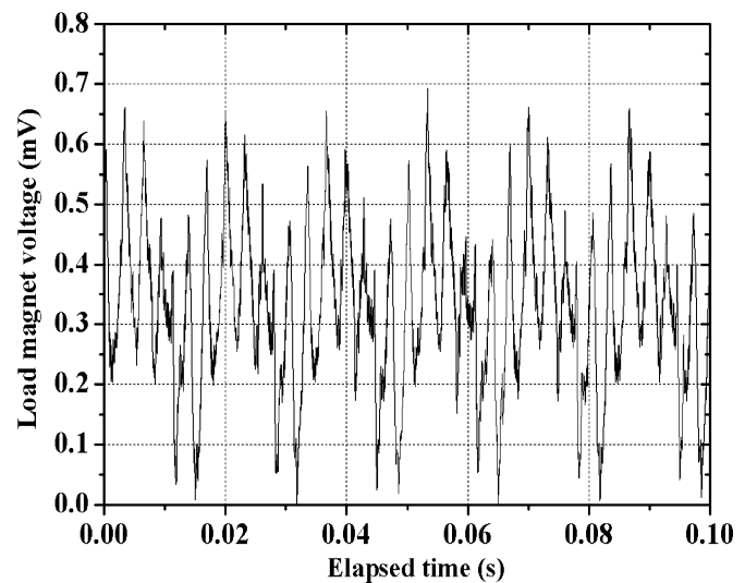
Fig. 8. Measured the load magnet voltage at 60 Hz.
