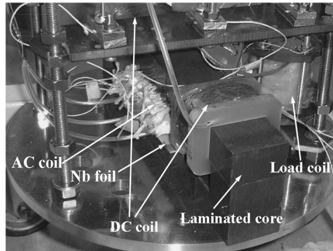
Fig. 5. Photograph of the linear type magnetic flux pump system.
