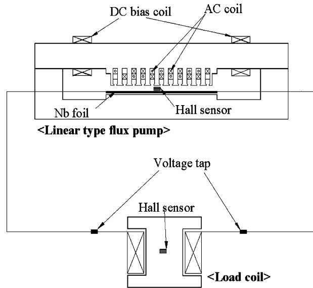
Fig. 4. Schematic diagram for the linear type flux pump system.
