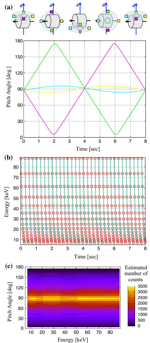
Fig. 2 a Variation of the pitch angle at the center of the field-of-view for sensor channels of the MEP-e during one spin period of 8 s under the assumed condition. Schematics shown in the upper panel represent the FOV of each sensor channel every 2 s, where the color of rectangles corresponds to those of plotted lines. b Energy range measured by MEP-e during one spin period, where 16 energy steps are swept every 0.25 s. c Estimated number of counts measured by the MEP-e during one spin period
