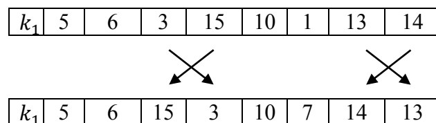
Figure 3.4 Mutation
