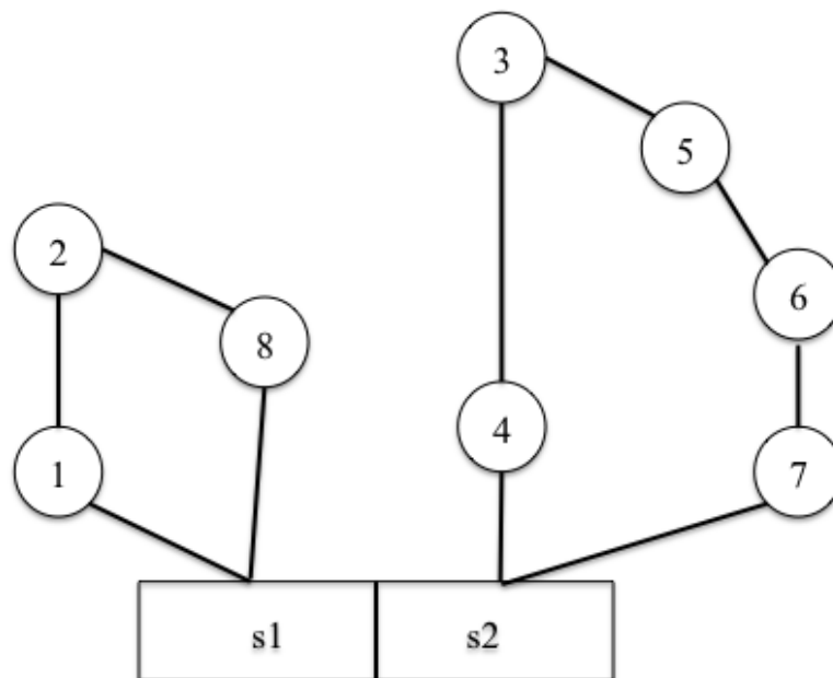
(b) Chromosome representative after crossover
