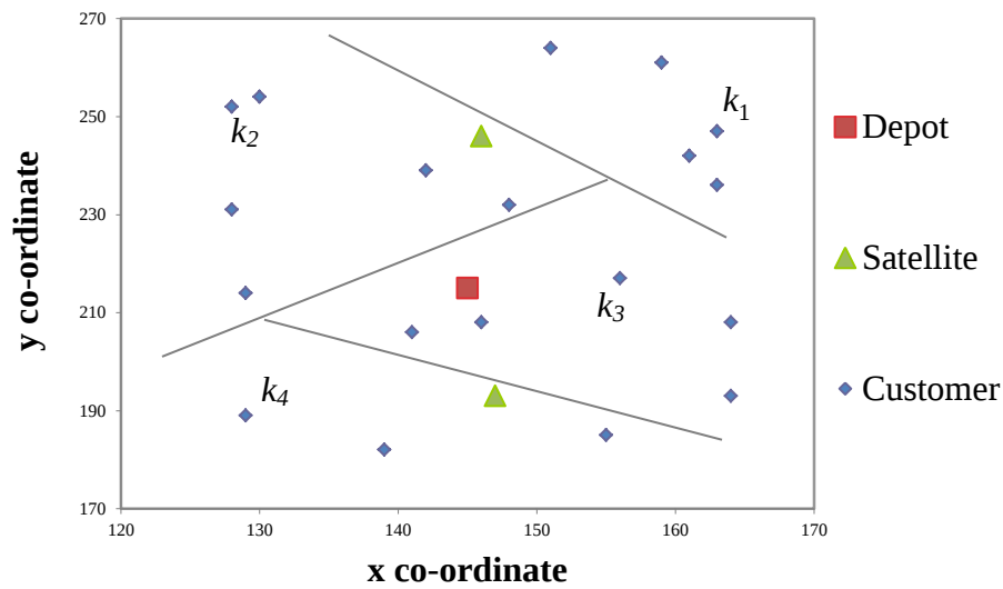
Figure 3.2 The clustered customers after k -means clustering
