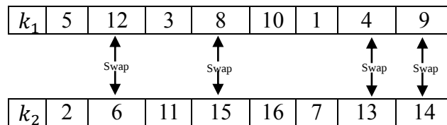
Figure 3.3 Uniform crossover
