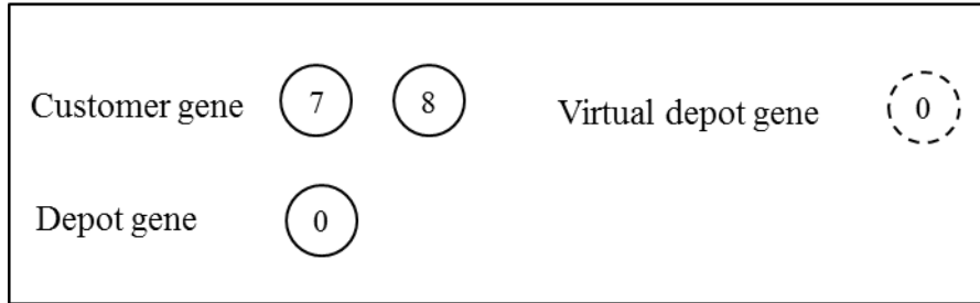
Figure 4.2 VRPTW chromosomes coding in GA-2
