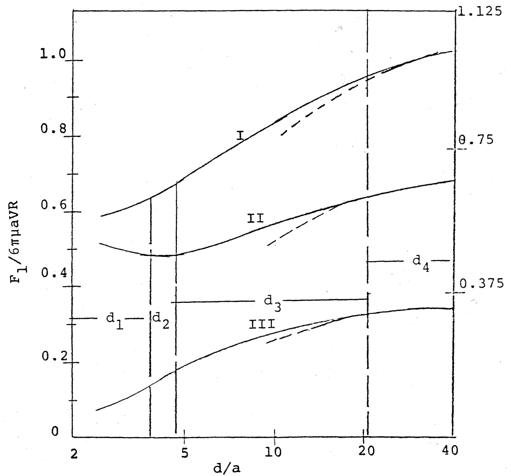
Fig.1 First-order force verses seperation
