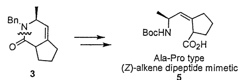
Scheme 1. Transformation of 3 to desired mimetic 5.
