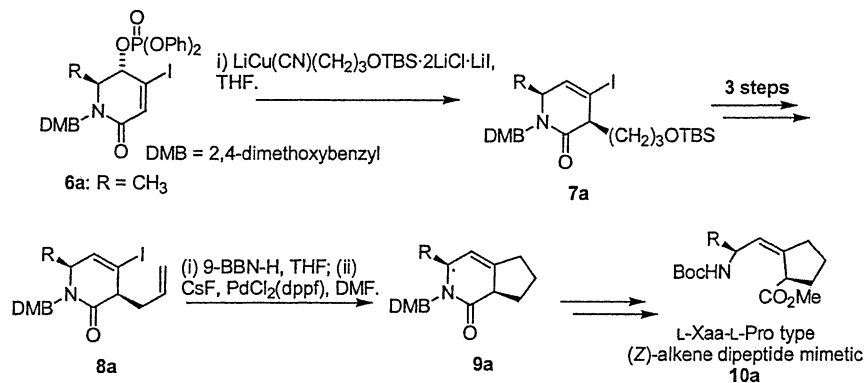
Scheme 2. Diastereoselective synthesis of Pro mimetics with organocopper reagents
