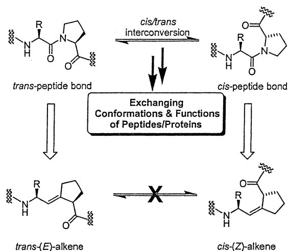
Figure 1. cis / trans -Interconversion of peptide bonds in Xaa-Pro dipeptides and their corresponding cis -( Z )-alkene or trans -( E )-alkene dipeptide isosteres.
