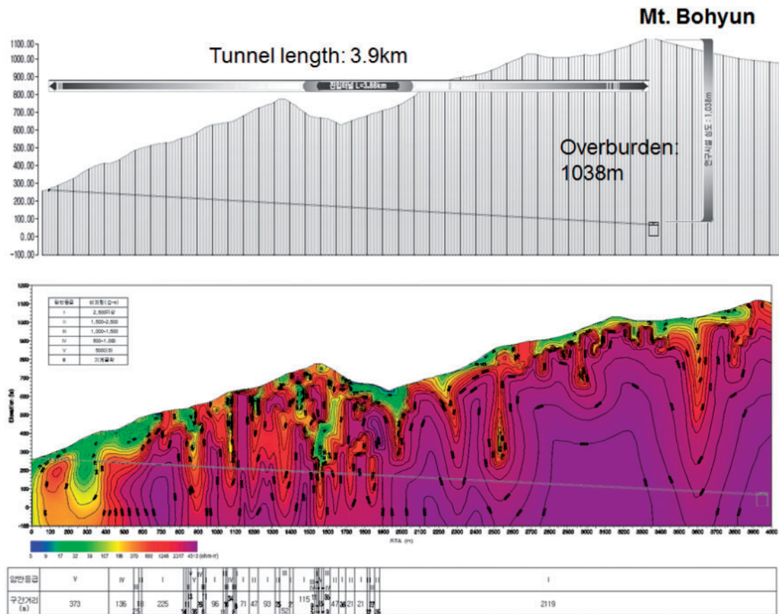
Fig. 5. Mount Bohyun as a candidate site for the second Hyper-K detector in Korea. It is 1124 m high and provides \sim 1000 m overburden with a slightly inclined access tunnel that is 3.9 km long. A geological survey shows excellent bedrock for the candidate site, suitable for a large cavern.
