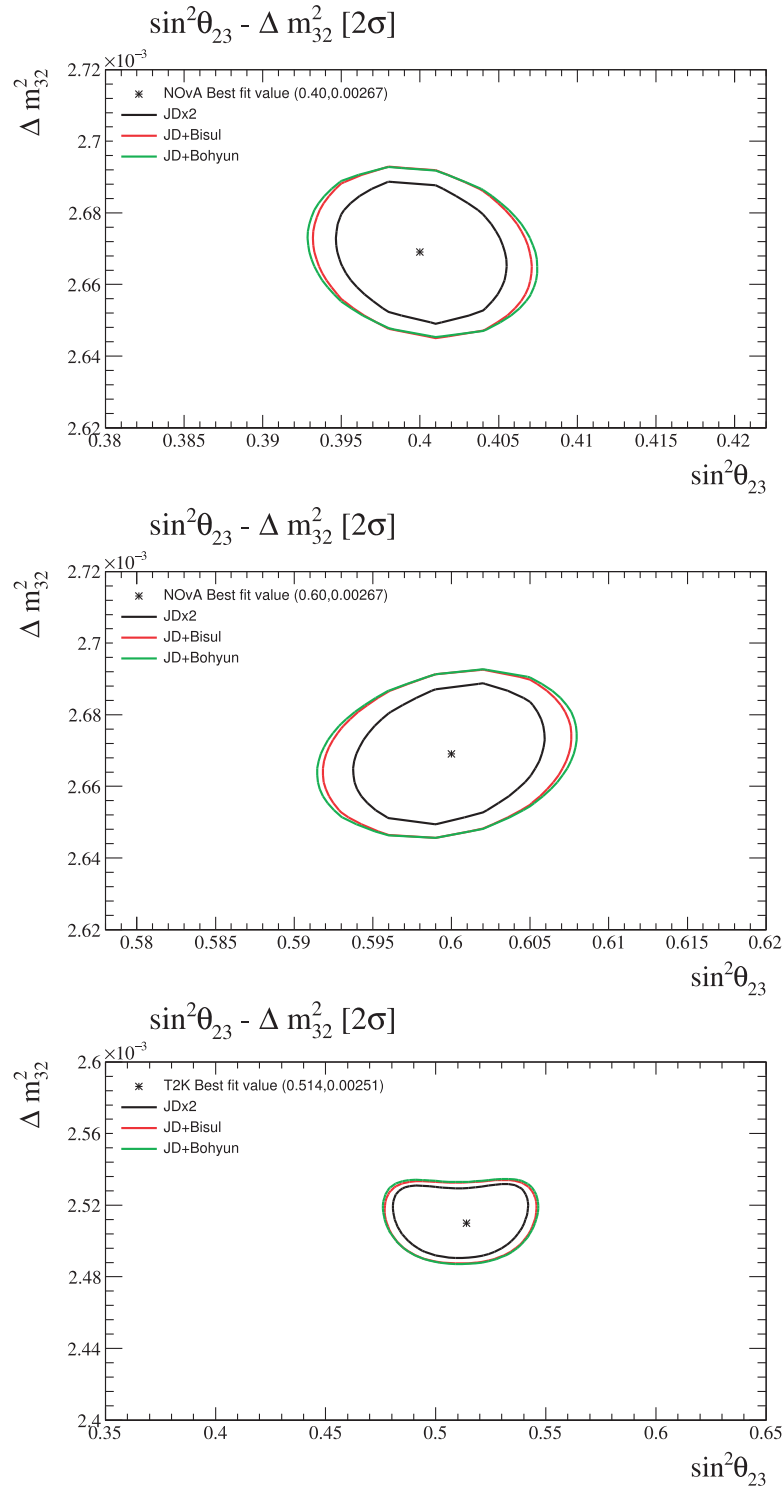
Fig.33. Two- \sigma sensitivity curves for the atmospheric parameter determination at true values of \Delta m^2_{32} = 2.67 \times 10^{-3} \text{ eV}^2 and \sin^2 \theta_{23} = 0.4 (top), \Delta m^2_{32} = 2.67 \times 10^{-3} \text{ eV}^2 and \sin^2 \theta_{23} = 0.6 (middle), \Delta m^2_{32} = 2.51 \times 10^{-3} \text{ eV}^2 and \sin^2 \theta_{23} = 0.514 (bottom).
