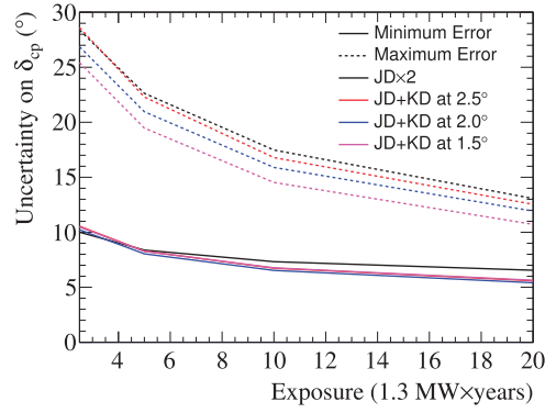
Fig. 29. The evolution of the \delta_{\text{CP}} measurement precision with exposure. The “Minimum” and “Maximum” errors are the uncertainties at the true \delta_{\text{CP}} and mass ordering values with the best and worst measurement resolution, respectively.
