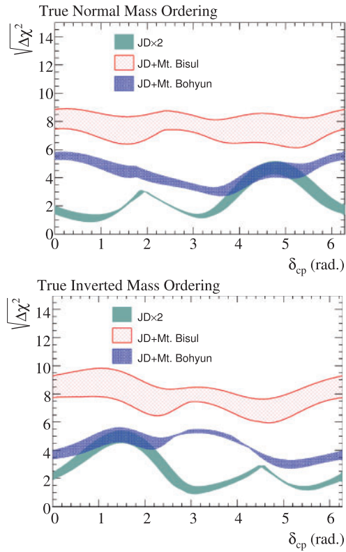
Fig. 30. The significance for the wrong mass ordering rejection as a function of the true value of \delta_{\text{CP}} and the true mass ordering (top=normal, bottom=inverted). Results are shown for the Mt. Bisul and Mt. Bohyun sites. The bands represent the dependence of the sensitivity on the true value of \sin^2 \theta_{23} in the range 0.4 < \sin^2 \theta_{23} < 0.6 .
