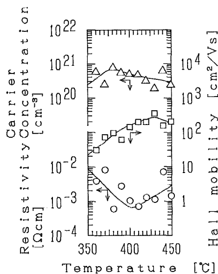
FIG. 4. Electric resistivity, carrier concentration, and Hall mobility for \text{In}_2\text{O}_3 :F film as a function of reaction temperature.
