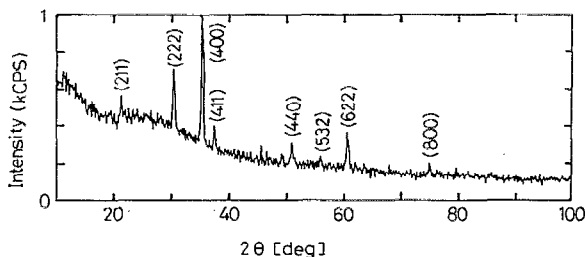
FIG. 1. X-ray diffraction patterns of the \text{In}_2\text{O}_3:\text{F} film deposited on borosilicate glass substrate at 380 °C.
