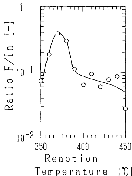
FIG. 5. The ratio F/In of \text{In}_2\text{O}_3 :F film as a function of reaction temperature.
