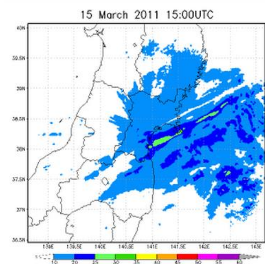
Fig. 4 An example of reflectivity of Japan Meteorological Agency C-band radar [23:50 -24:00 JST, 15 March, 2 km height, unit: dBZ] .
