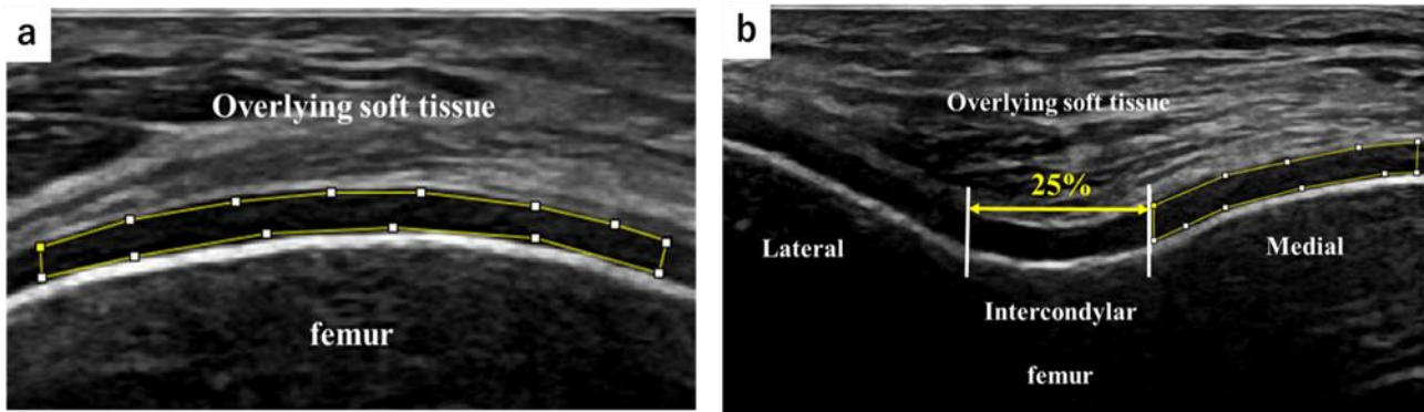
317 Fig. 1 Ultrasonographic image of the femoral cartilage
