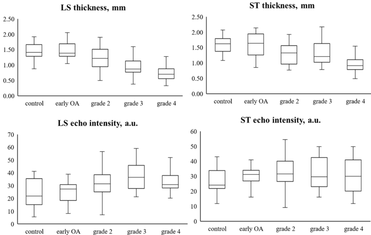
324 Fig. 2 Unadjusted thickness and echo intensity of the femoral medial cartilage in each group
