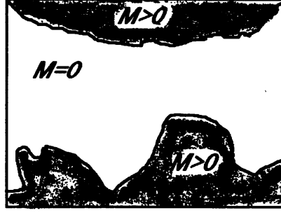
Fig. 1: Schematic sketch of the biofilm model setup. The actual biofilm is the biomass occupied region \Omega_2(t) = \{x \in \Omega \mid M(t, x) > 0\} the region \Omega_1(t) = \{x \in \Omega \mid M(t, x) = 0\} without biomass represents the liquid region.
