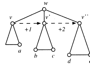
\overline{\mathcal{P}_k}
