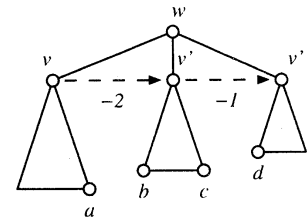
\mathcal{P}_k
