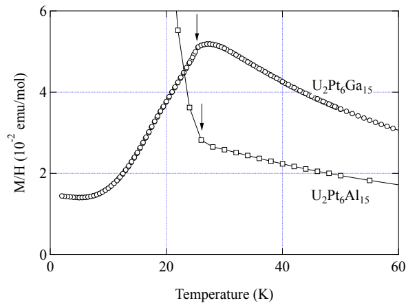
Figure 1. Temperature dependence of magnetization divided by magnetic field for \text{U}_2\text{Pt}_6\text{Al}_{15} and \text{U}_2\text{Pt}_6\text{Ga}_{15} .
