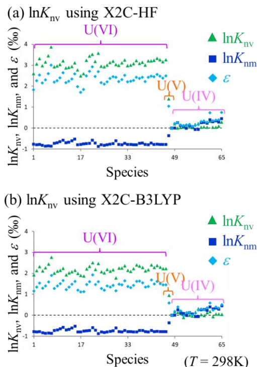
Fig. 1. \ln K_{\text{nv}} , \ln K_{\text{nm}} , and \varepsilon of 64 U species, calculated (a) at the HF level and (b) at the B3LYP levels for \ln K_{\text{nv}} . The light blue, green, and deep blue plots represent \varepsilon , \ln K_{\text{nv}} , and \ln K_{\text{nm}} , respectively. These plots for U(VI), U(V), and U(IV) species are surrounded by the purple, orange, and pink rounded squares, respectively. [8]
