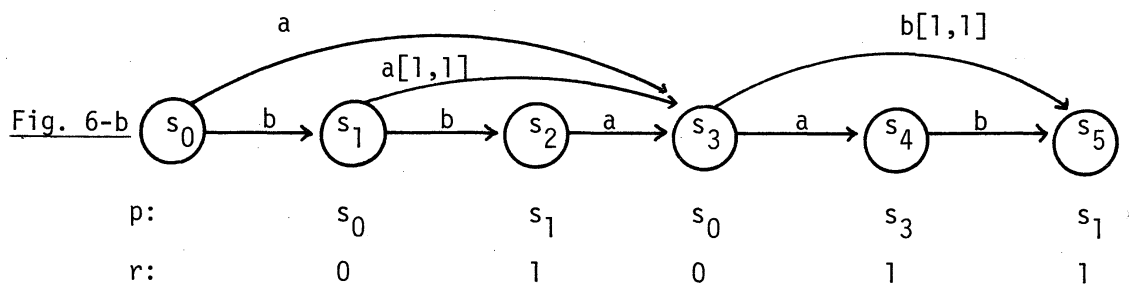
Fig. 6- Construction process of an SMM. (interval [0, \infty] is omitted)
