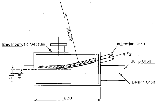
Fig. 5. Injection orbit.
