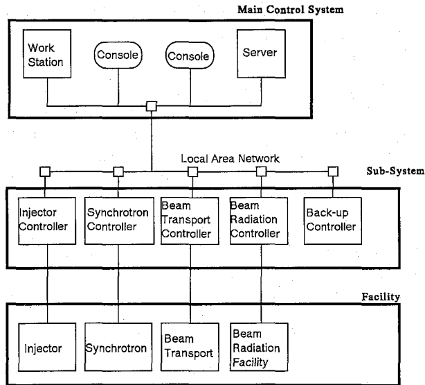
Fig. 14. Block diagram of the control system.
