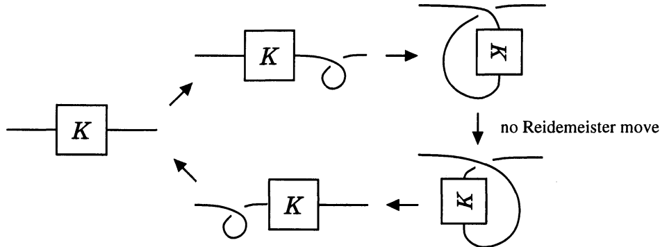
Figure 4: One realization of the loop \text{rot}(K) as a sequence of Reidemeister moves
