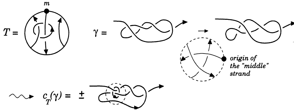
Figure 6: Elementary cochain associated with an oriented tangle T . The middle strand issue is explained in Subsection 2.1.3.
