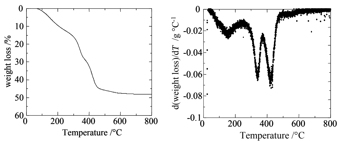
Fig. 4-2. Weight loss (left) and it differential profile (right) during the thermal analysis of the decyl derivative of boehmite in He.
