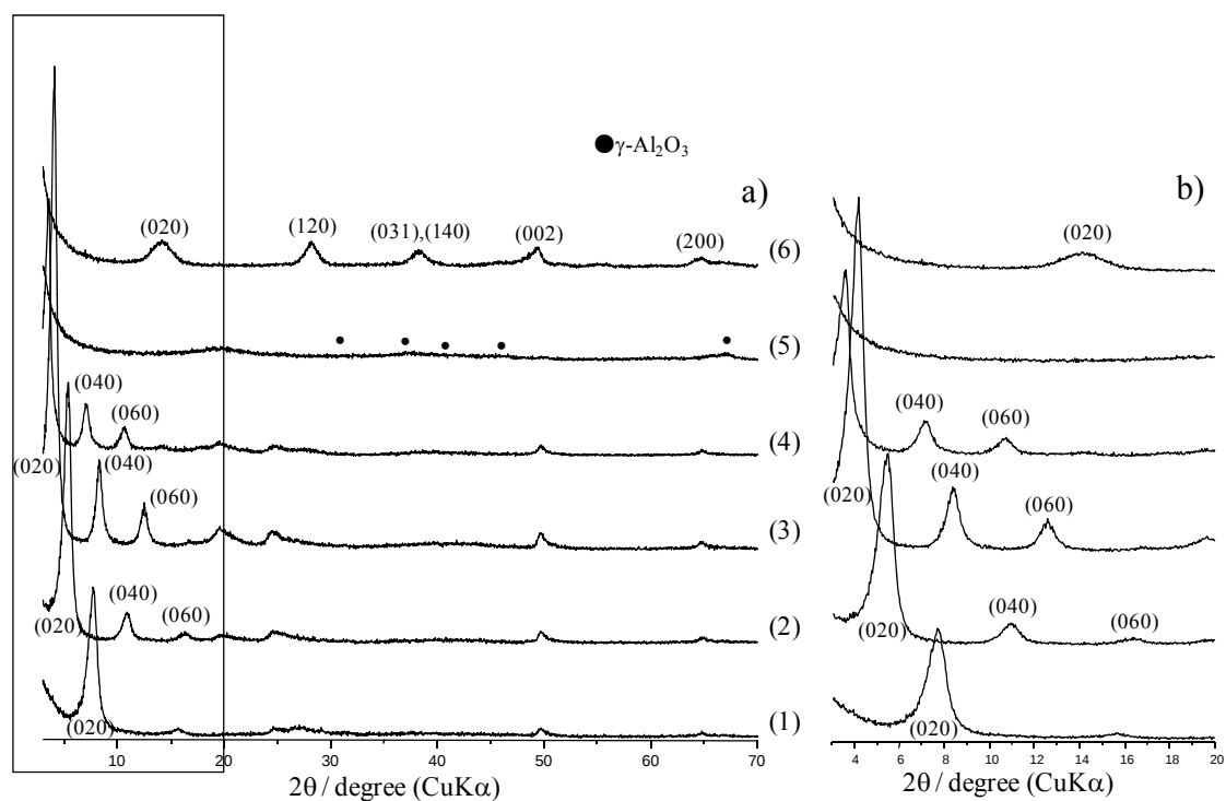
Fig. 2-1. X-ray diffraction patterns of the products recovered as xerogel/aerogel after solvothermal reaction of AIP in various alcohols: 1, AEtOH(assyn); 2, ABuOH(assyn); 3, AHeOH(assyn); 4, AOcOH(assyn); 5, ADDOH(assyn); 6, Pseudoboehmite.
