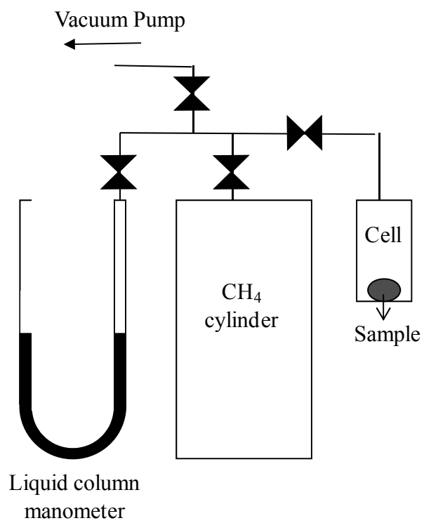
Fig. 4-1. Apparatus methane adsorption for measurement.
