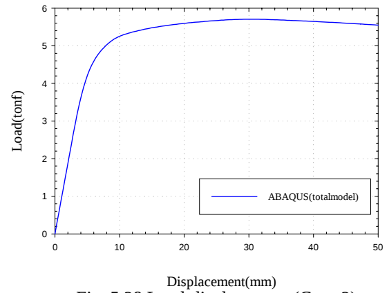
Fig. 5.28 Load-displacement (Case-2)
