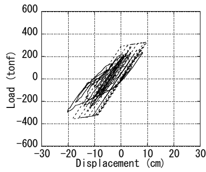
(b) Load-displacement (Analysis of system of particles)
