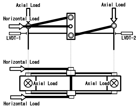
Fig. 4.2 Loading apparatus
