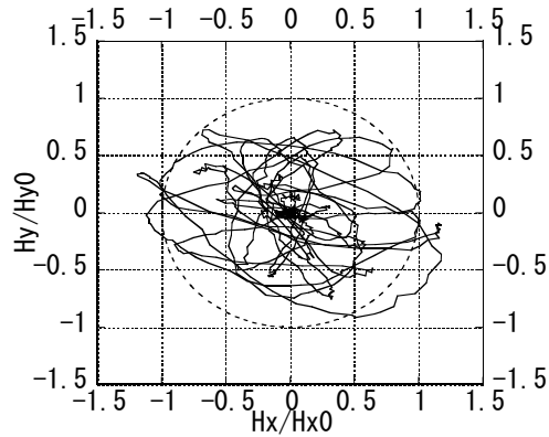
Fig. 5.20 Trajectory of the horizontal restoring forces in X and Y directions
