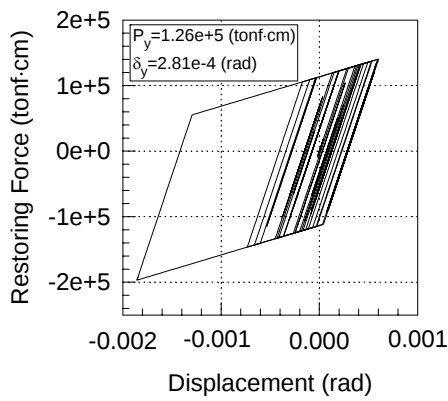
(b) Hysteretic curve
