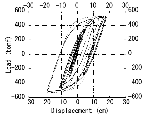
(c) Load-displacement
