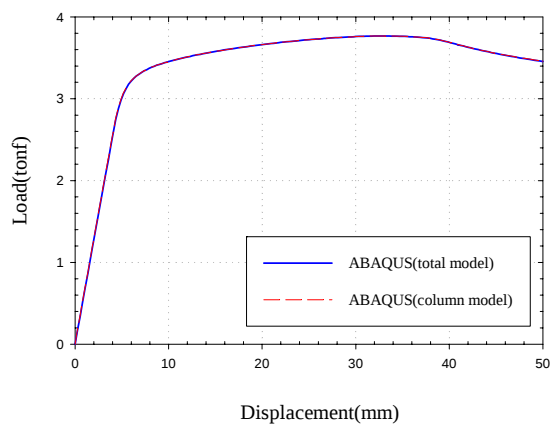
Fig. 5.31 Load-displacement (Case-5)
