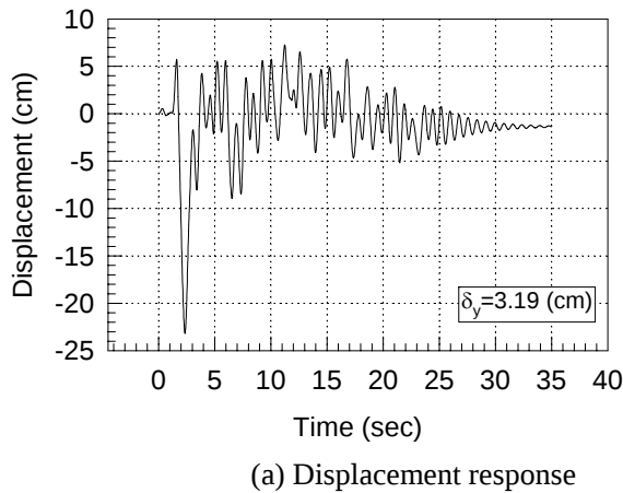
Fig. 3.5 Analytical results (Superstructure: Foundation is fixed)
