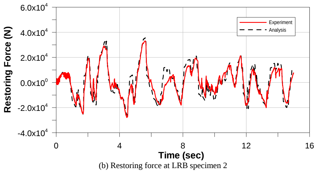
Fig. 6.32 Displacement response and restoring force of bearing specimen: LRB 2
