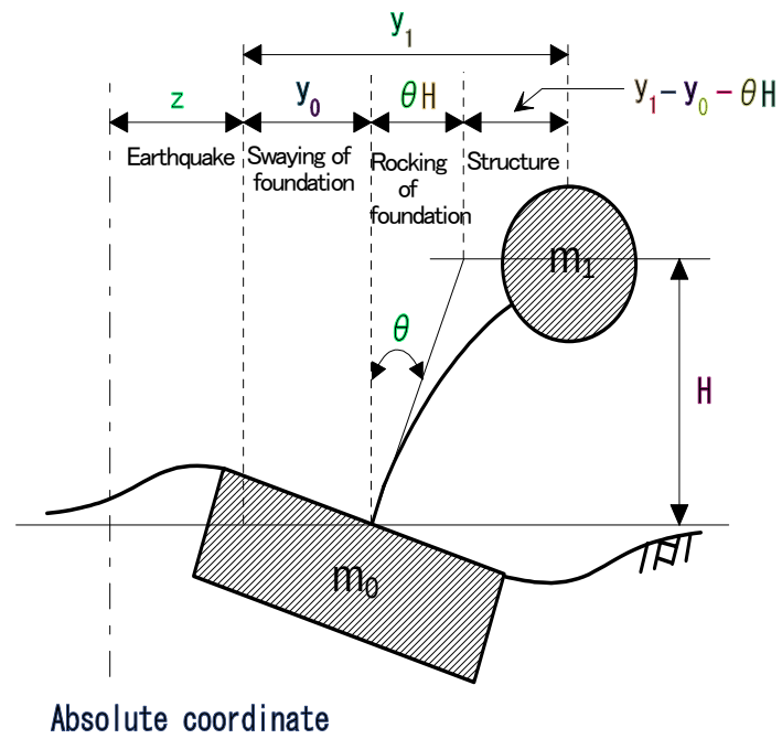
Fig. 3.1 Modeling of structure-foundation system
