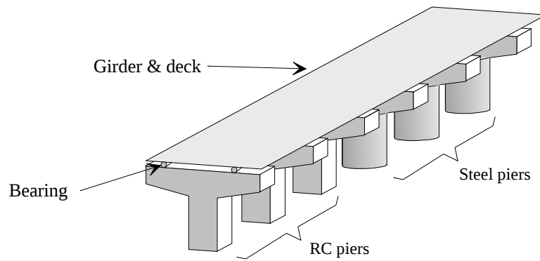
Fig. 2.1 Elevated bridge system consisting of steel and RC piers
