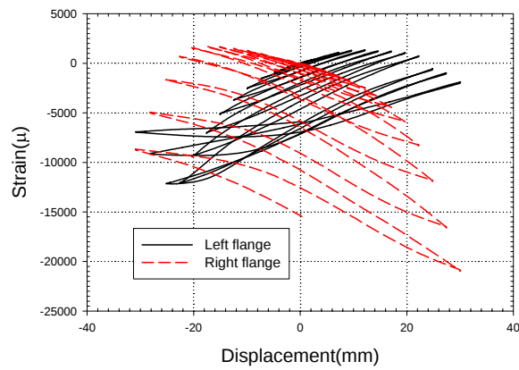
Fig. 4.15 Axial strain (Flange plate in left column)
