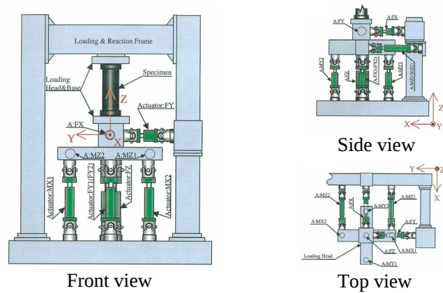
Fig. 5.2 Loading apparatus
