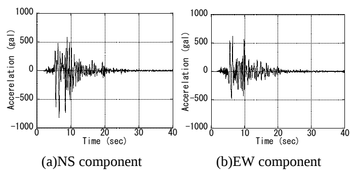
Fig. 5.4 Seismic wave observed at the Kobe marine meteorological observatory
