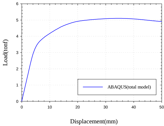
Fig. 5.29 Load-displacement (Case-3)
