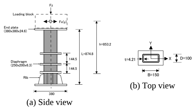
Fig. 5.1 Specimen (unit: mm)
