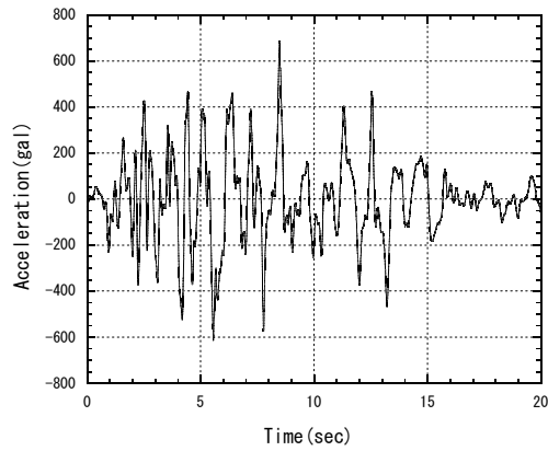
Fig. 6.21 Ground motion
