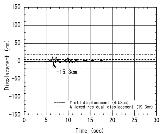
Fig. 4.18 Displacement response (Input acceleration 1: 1 time)
