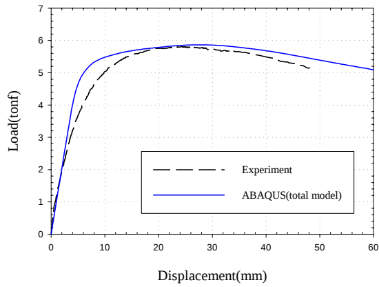
Fig. 5.27 Load-displacement (Case-1)
