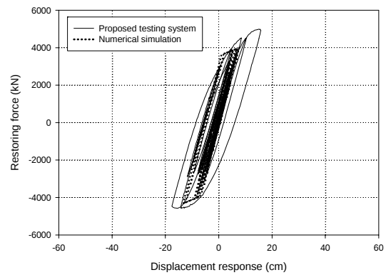
(b) Restoring force vs. displacement response
