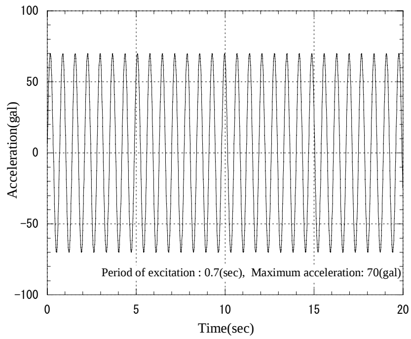
Fig. 6.4 Ground motion
