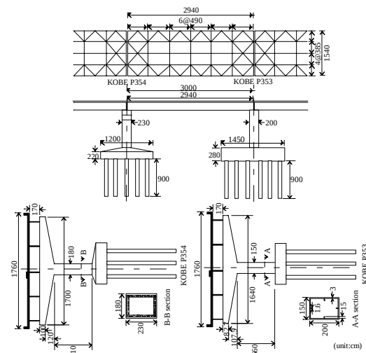
Fig. 2.2 Existing elevated bridge (Hanshin Expressway (Kobe route))
