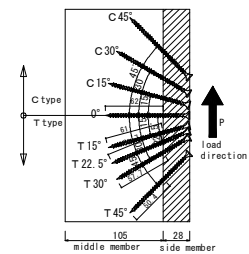
Figure 2. Inclination angle of screws
