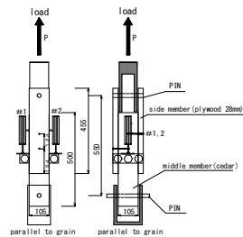
Figure 1. Tensile test setup
