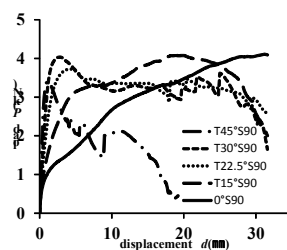
Figure 3. Load- deformation curves of T type specimens
