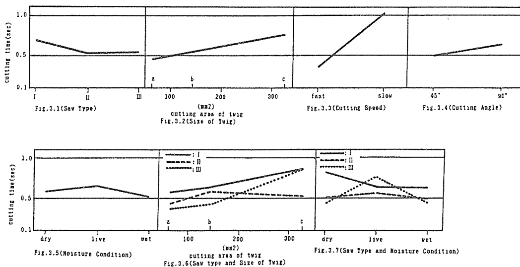
Fig. 3 Cutting time on each factorial effect
