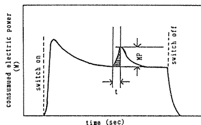
Fig. 2 Chart of the auto pen-recorder about the consumed electric power with a circular saw t: cutting time MP: maximum instantaneous consumed electric power
