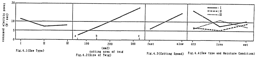
Fig. 4 Consumed electric power on each factorial effect
