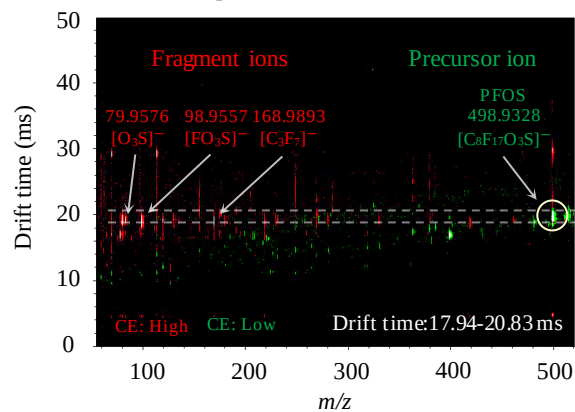
(b-1): PFOS in a sample (G5) (RT:5.302-5.514 min)
