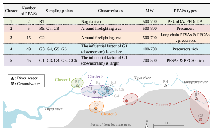
Fig. 7.1 Summary of this study
