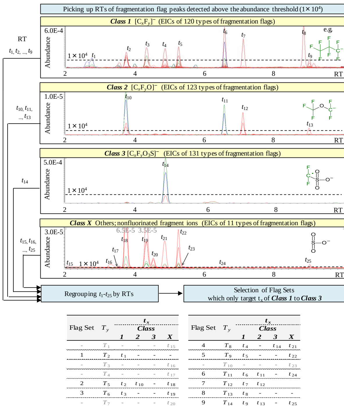
Fig. 6.5 Selection of peaks by fragmentation flagging for a fire extinguisher liquid. The EICs were described at 10 V in blue, 20 V in green, and 40 V in red.
