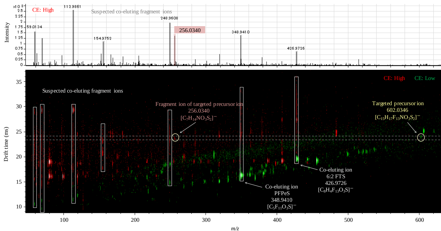
Fig. 5.6 The mass spectrum at a specific RT with drift time for targeted [C_{15}H_{17}F_{13}NO_3S_2]^- ( m/z 602.0346) in a groundwater sample (G5)
