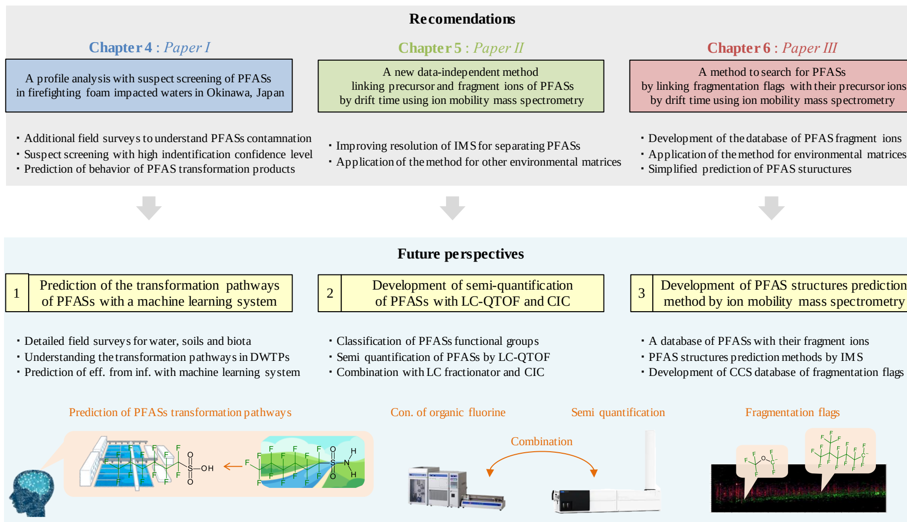
Fig. 7.2 Recomendations and future perspectives
