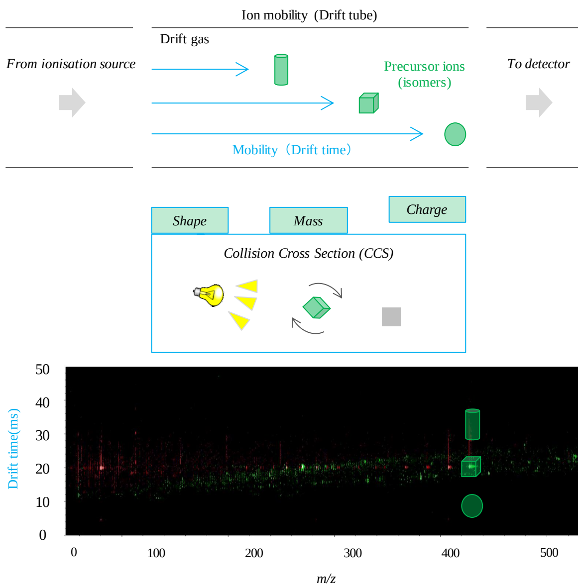
Fig. 2.5 Separation of precursor ions (e.g. isomers) by ion mobility mass spectrometry (Borsdorf et al., 2006; Creaser et al., 2004; Lanucara et al., 2014)
