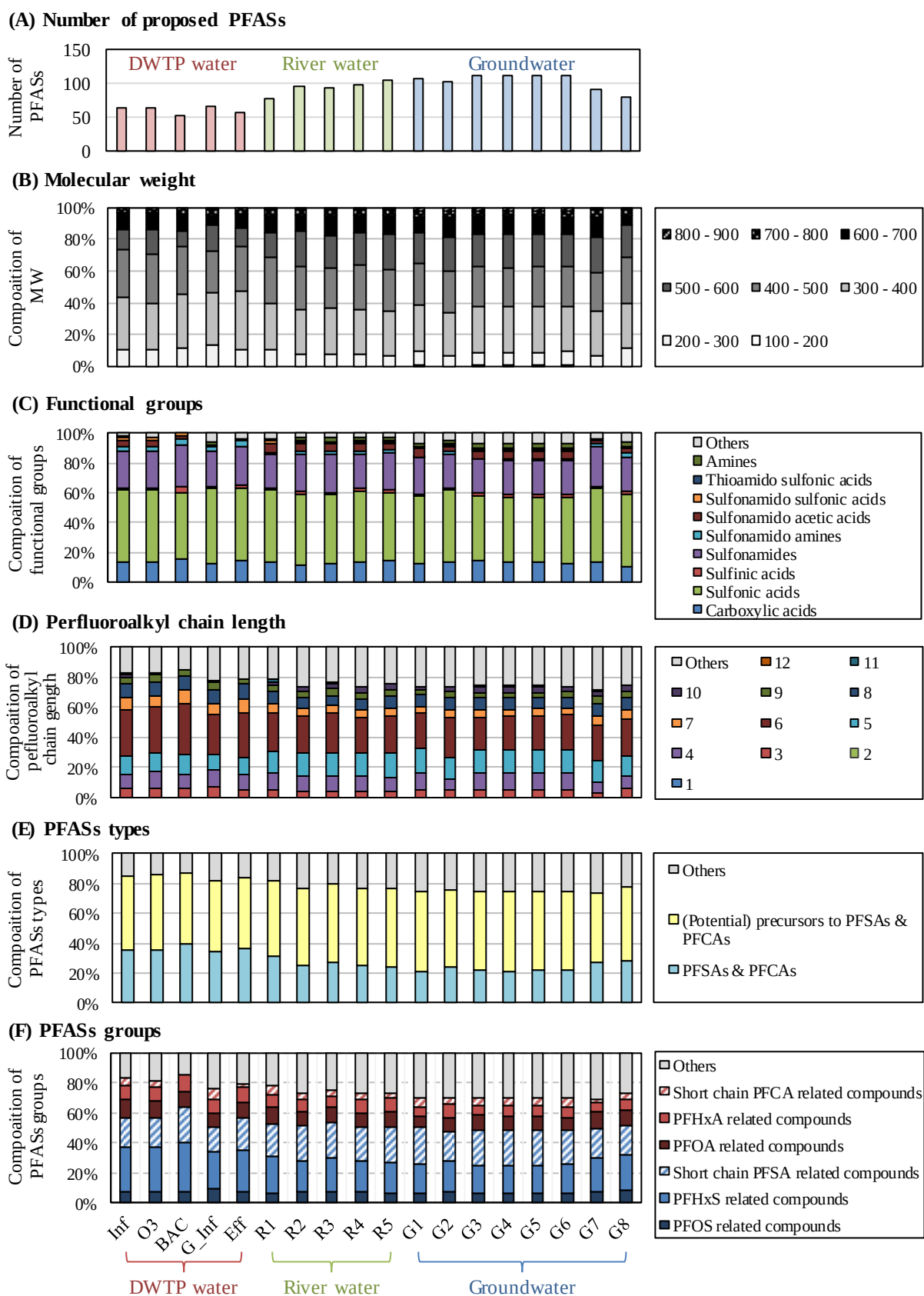
Fig. 4.3 (A) Numbers of proposed PFASs (peak areas > 10 000) in firefighting foam impacted waters. (B–F) Profiles of proposed PFASs by (B) molecular weight, (C) functional group, (D) perfluoroalkyl chain length, (E) PFAS type, (F) PFAS group.
