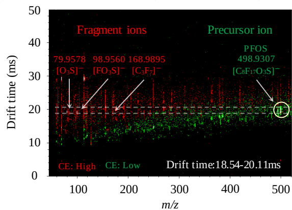
(a-1): PFOS in STD mixture (RT:5.359-5.494 min)
