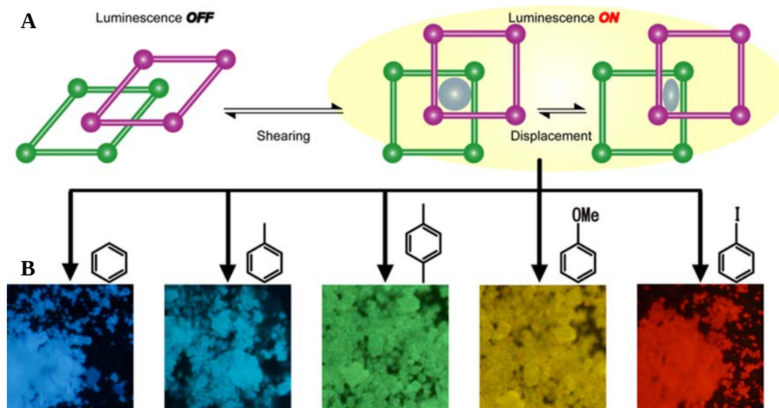
Figure 2. (A) Structural dynamics of the MOF on the accommodation of different guest molecules. (B) fluorescence image of [Zn 2 (bdc) 2 (dpNDI)] n powder with different VOC (Volatile Organic Compounds) molecules occluded in the pore: benzene, toluene, p -xylene, anisole and iodobenzene.
