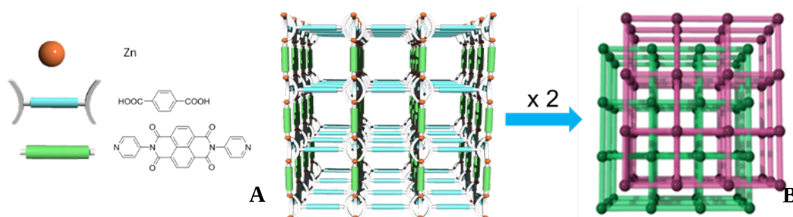
Figure 1. (A) Illustrative representation of one of the two identical frameworks that compose the [\text{Zn}_2(\text{bdc})_2(\text{dpNDI})]_n MOF indicating its different components; (B) an schematic representation of the interpenetration of the two identical frameworks.
