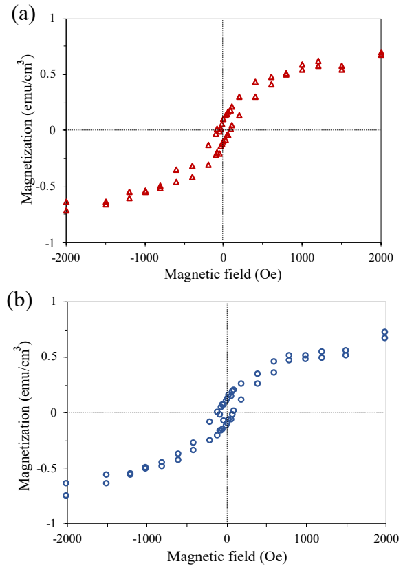
Fig. 6. Magnetization versus applied magnetic field curves measured at 300 K for the (a) epitaxial and (b) polycrystalline Mn-doped ITO films.
