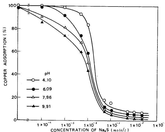
Fig. 1. Relationship between the copper adsorption on sphalerite and the concentration of sodium sulphide.
