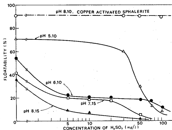
Fig. 8. Effect of sulphurous acid on the floatability of sphalerite when copper activation of sphalerite is prevented by sodium sulphide.
