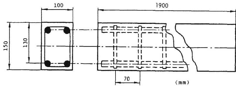
Figure 3.1 Specimen dimensions.
