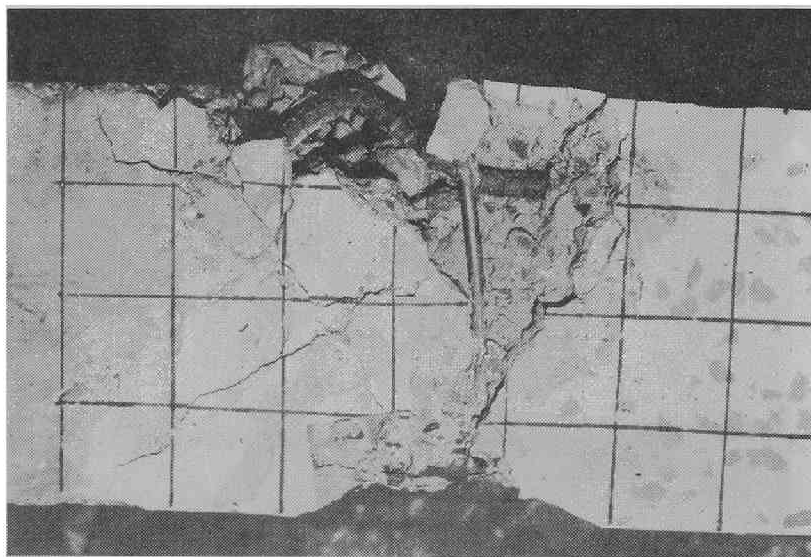
Photo 3.9 Crushed segment of No. 8 specimen.
