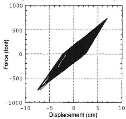
(c) Strengthened with 2 mm steel jackets
