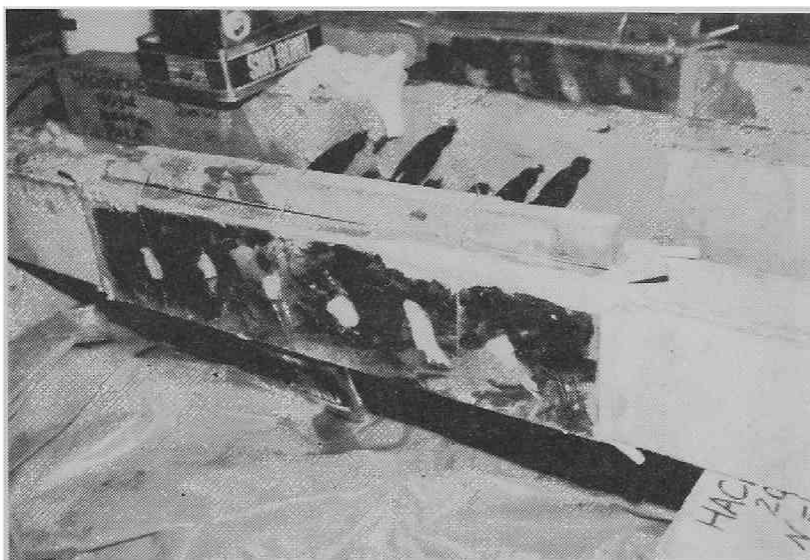
Photo 3.6 Type III repair: Setting steel plates around the specimen.
