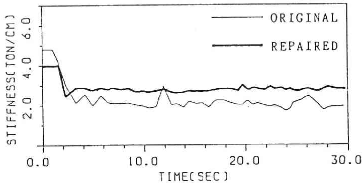
(b) Specimen 7 (El Centro, 250 gal. Repaired with the epoxy resin grouting method; Type I)
