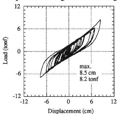
(3) Girder (above HDR) hysteretic response during main loading.
