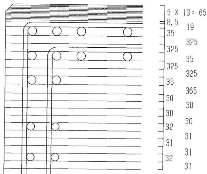
Figure 4.14 (b) Discrete fiber elements for a cross section of the pier above the termination point of the reinforcing bars.
