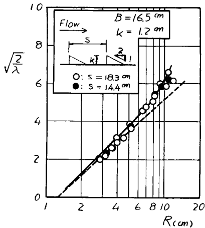
Fig. 5 Variation of frictional factor \sqrt{2/\lambda}
