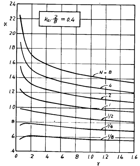
Fig. 3 Relation between \alpha and \gamma for different values of N and 2k_{s1}/B
