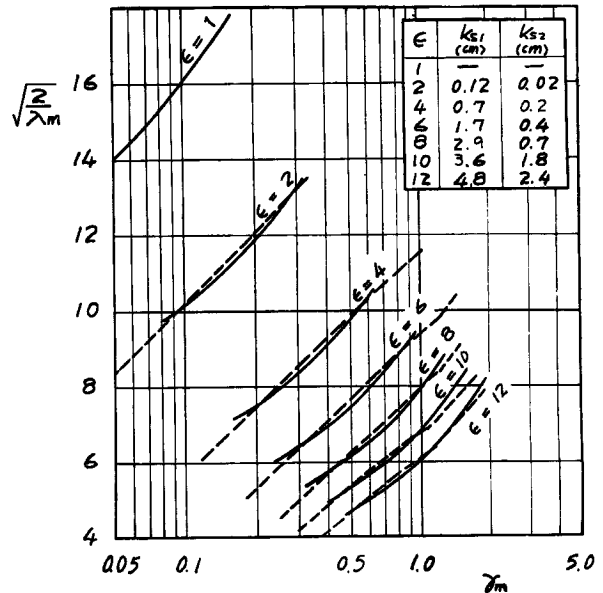
Fig. 8 Conditions of similitude (horizontal scale : 1/500, n_p : 0.035 , B_p : 60 \text{ meters} )
