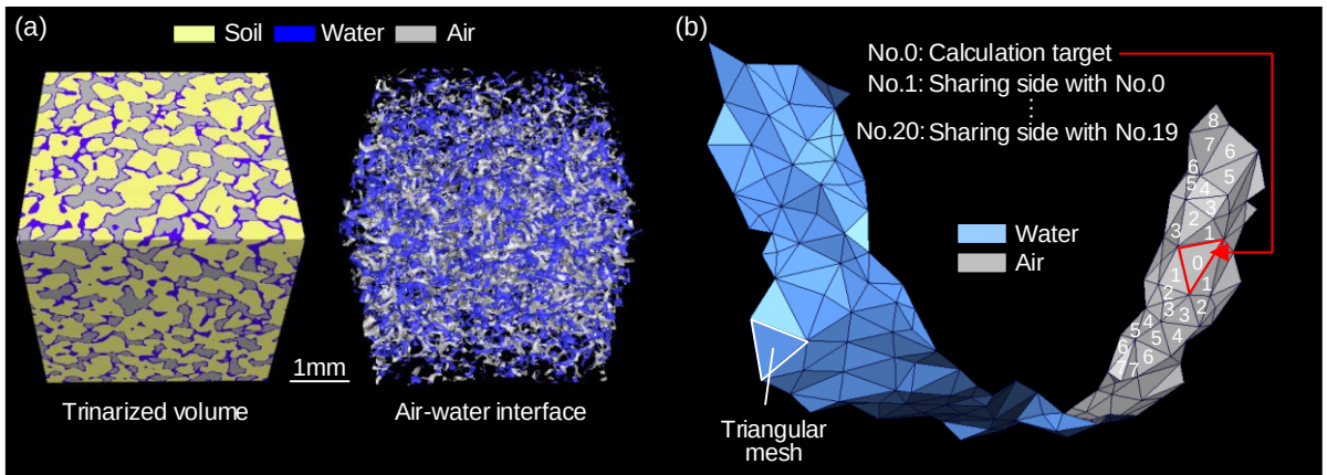
Fig. 8 a air-water interface extracted from trinarized volume and b triangular meshes and principle of considering neighborhood of calculation target
