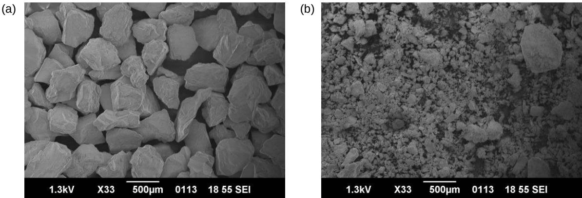
Fig. 1 SEM images: a silica sand (poorly-graded sand) and b Yodogawa sand (well-graded sand)
