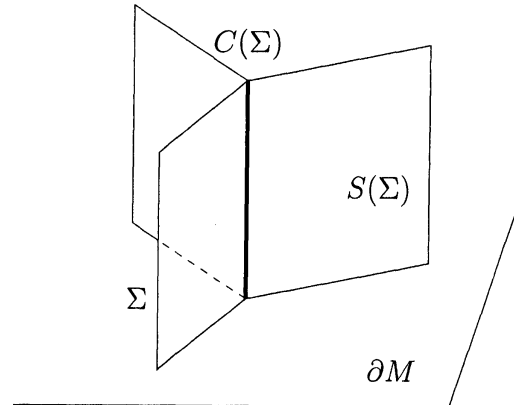
A tribranched Surface \Sigma (local picture)
