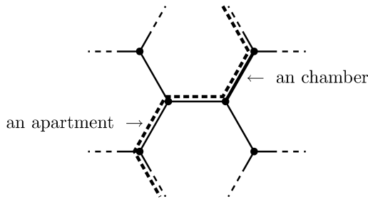
The Bruhat-Tits tree as an Euclidean building
