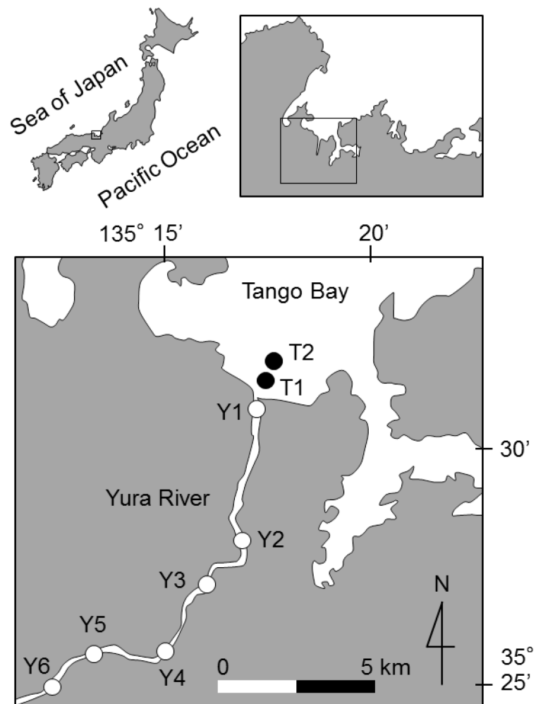
Fig. 2-1. Yura River estuary and study sites, including river stations (○) and coastal stations (●).
