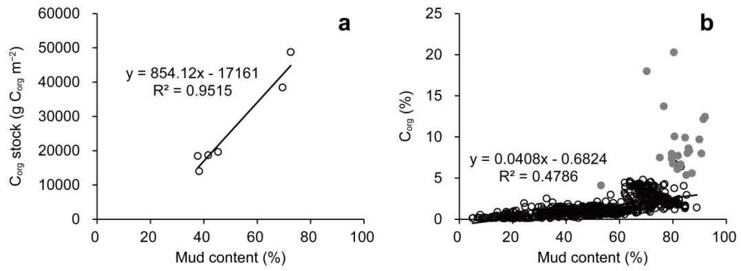
Fig. 6-8. (a) The relationship between mean mud ( < 63 \mu\text{m} fraction) contents and 2 m C_{org} stocks in six sediment cores. (b) The relationship between mud contents and C_{org} concentrations in each sample. Closed gray circles show the samples taken from peaty layers.
