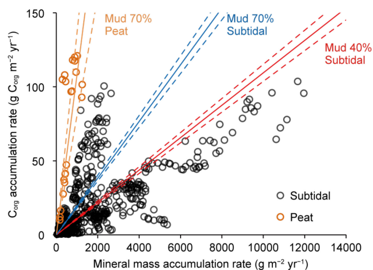
Fig. 6-9. Relationships between organic carbon ( C_{org} ) accumulation rate, mineral mass accumulation rate, mud ( <63\ \mu m ) content, and sediment type (peat/subtidal) analyzed with a generalized linear model. The solid and dashed lines indicate the linear models and their 95% confidence intervals, respectively.
