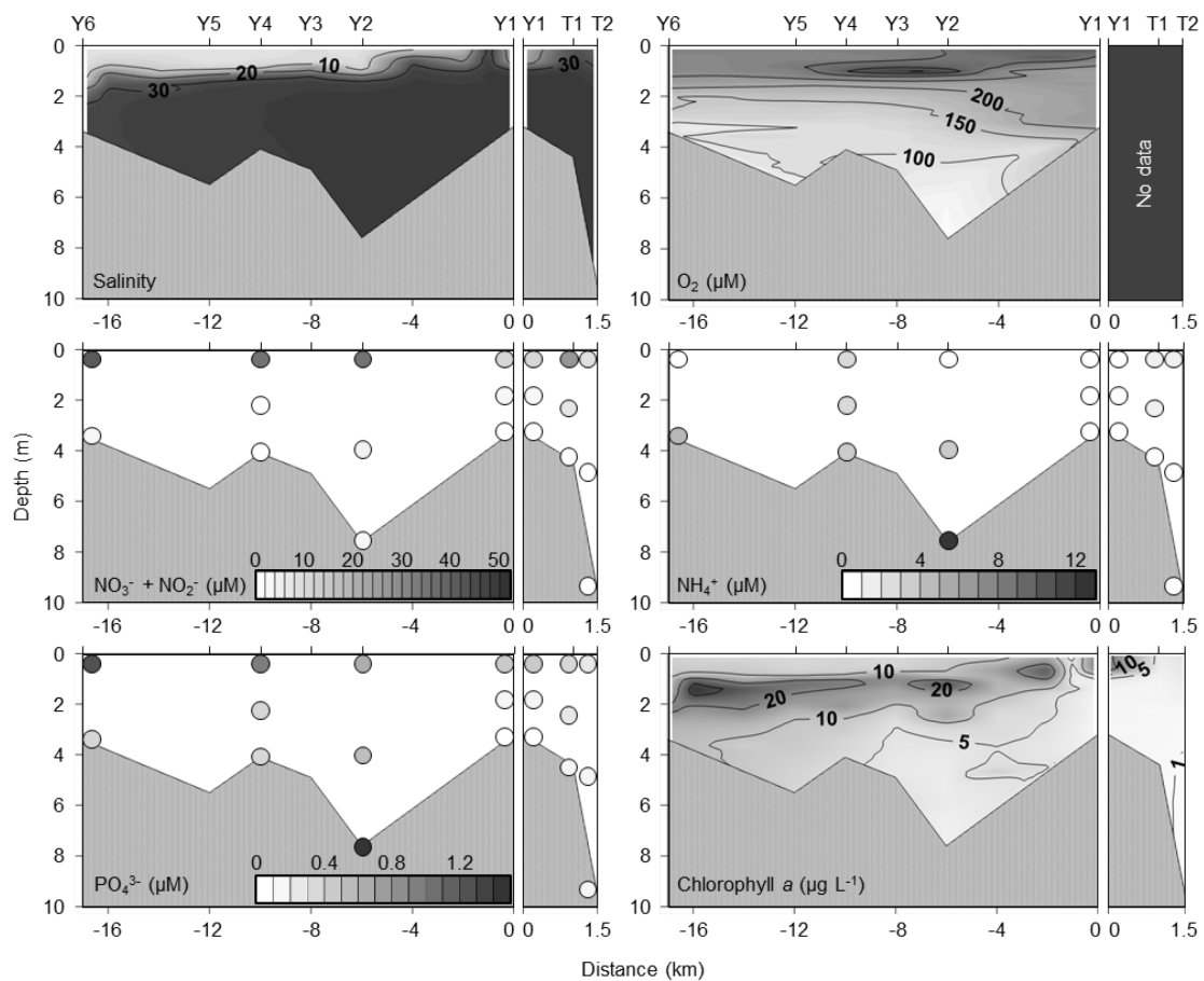
Fig. 2-3. Longitudinal transects of salinity, dissolved oxygen ( \text{O}_2 ), \text{NO}_3^- + \text{NO}_2^- , \text{NH}_4^+ , \text{PO}_4^{3-} , and chlorophyll a along the Yura River estuary on 22–23 August 2007.
