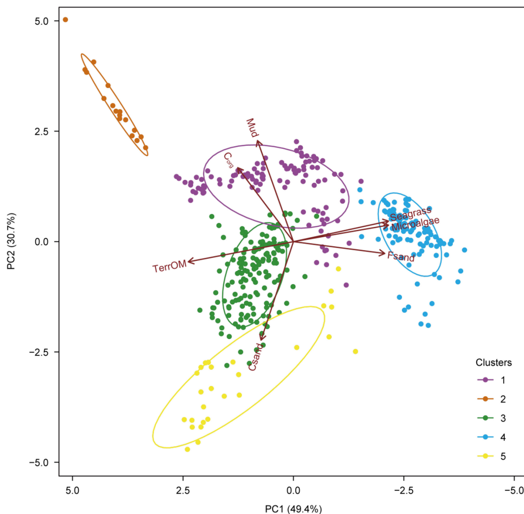
Fig. 6-10. Principal component analysis of C_{org} concentration, grain-size composition ( C_{sand} , >500\ \mu m ; F_{sand} , 63\text{--}500\ \mu m ; Mud , <63\ \mu m ), and C_{org} source composition of the sediment samples identified by the change point analysis. The first two axes accounted for 80.1% of the variance. TerrOM, terrestrial-derived organic matter.
