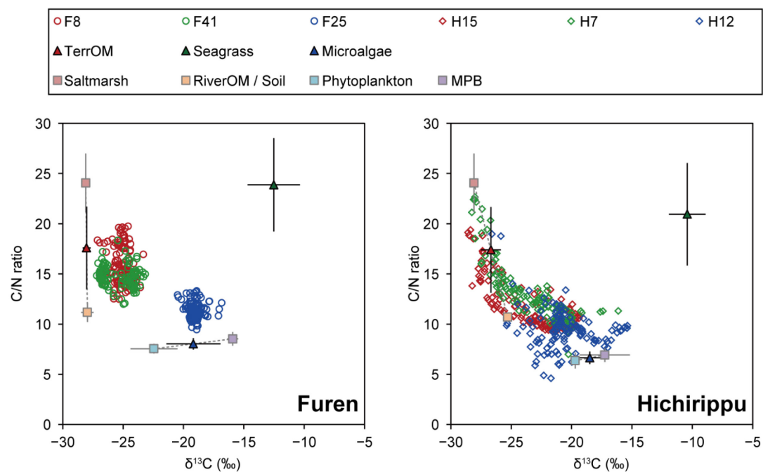
Fig. 6-2. Isotopic and elemental signatures of C_{org} sources and sediment samples in Furen and Hichirippu lagoons. Error bars represent standard deviations of each source.
