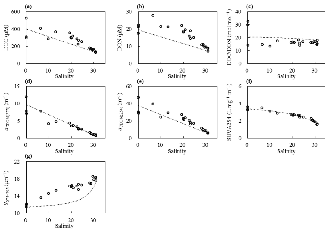
Fig. 5-3. Variations in concentrations of (a) DOC and (b) DON, (c) molar DOC/DON ratio, (d) a_{\text{CDOM}(375)} , (e) a_{\text{CDOM}(254)} , (f), SUVA 254 and (g) S_{275-295} along the salinity gradient in the Furen Lagoon. Dashed lines indicate the predicted conservative mixing relationships.
