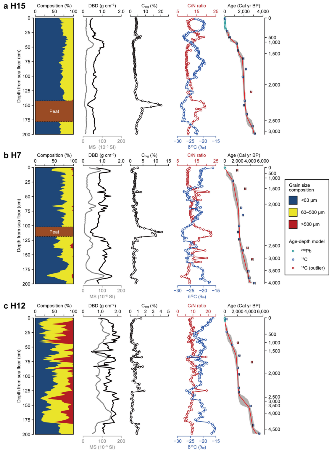
Fig. 6-5. Vertical profiles of grain size composition, dry bulk density (DBD), magnetic susceptibility (MS), organic carbon (C org ) concentration, C/N ratio, δ 13 C, and age–depth model at sampling sites in Hichirippu Lagoon. In the age–depth model, the red lines and gray areas represent the weighted mean estimates and 95% confidence intervals.
