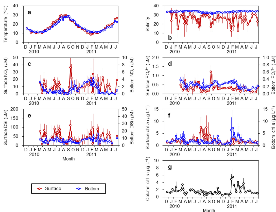
Fig. 3-2. Temporal changes in mean (a) temperature ( ^{\circ}\text{C} ), (b) salinity, (c) \text{NO}_x ( \mu\text{M} ), (d) \text{PO}_4^{3-} ( \mu\text{M} ), (e) DSi ( \mu\text{M} ), (f) chl a ( \mu\text{g L}^{-1} ) and (g) column chl a concentration ( \mu\text{g L}^{-1} ) of stations T1–T4 in Tango Bay. Red and blue circles indicate means of surface and bottom waters, respectively. The scales for the surface and bottom nutrient concentrations are different. Column chl a concentrations are water column means. Error bars indicate \pm standard deviations of the mean values ( n=4 ).
