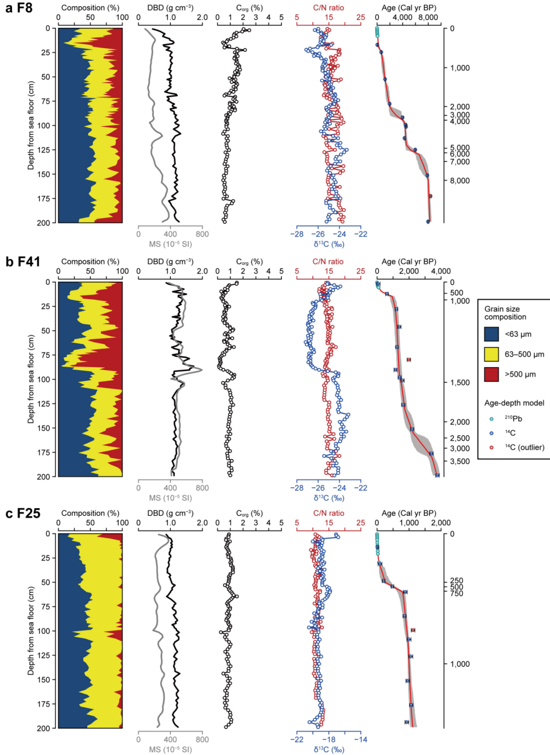
Fig. 6-4. Vertical profiles of grain size composition, dry bulk density (DBD), magnetic susceptibility (MS), organic carbon (C org ) concentration, C/N ratio, δ 13 C, and age–depth model at sampling sites in Furen Lagoon. In the age–depth model, red lines and gray areas represent the weighted mean estimates and 95% confidence intervals.
