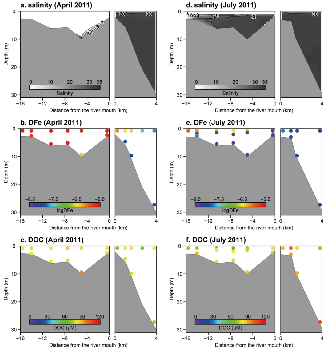
Fig. S4-3. Spatial distributions of salinity, dissolved iron (DFe), and dissolved organic carbon (DOC) concentrations in (a–c) April 2011 and (d–f) July 2011. The DFe concentration is represented as logDFe.
