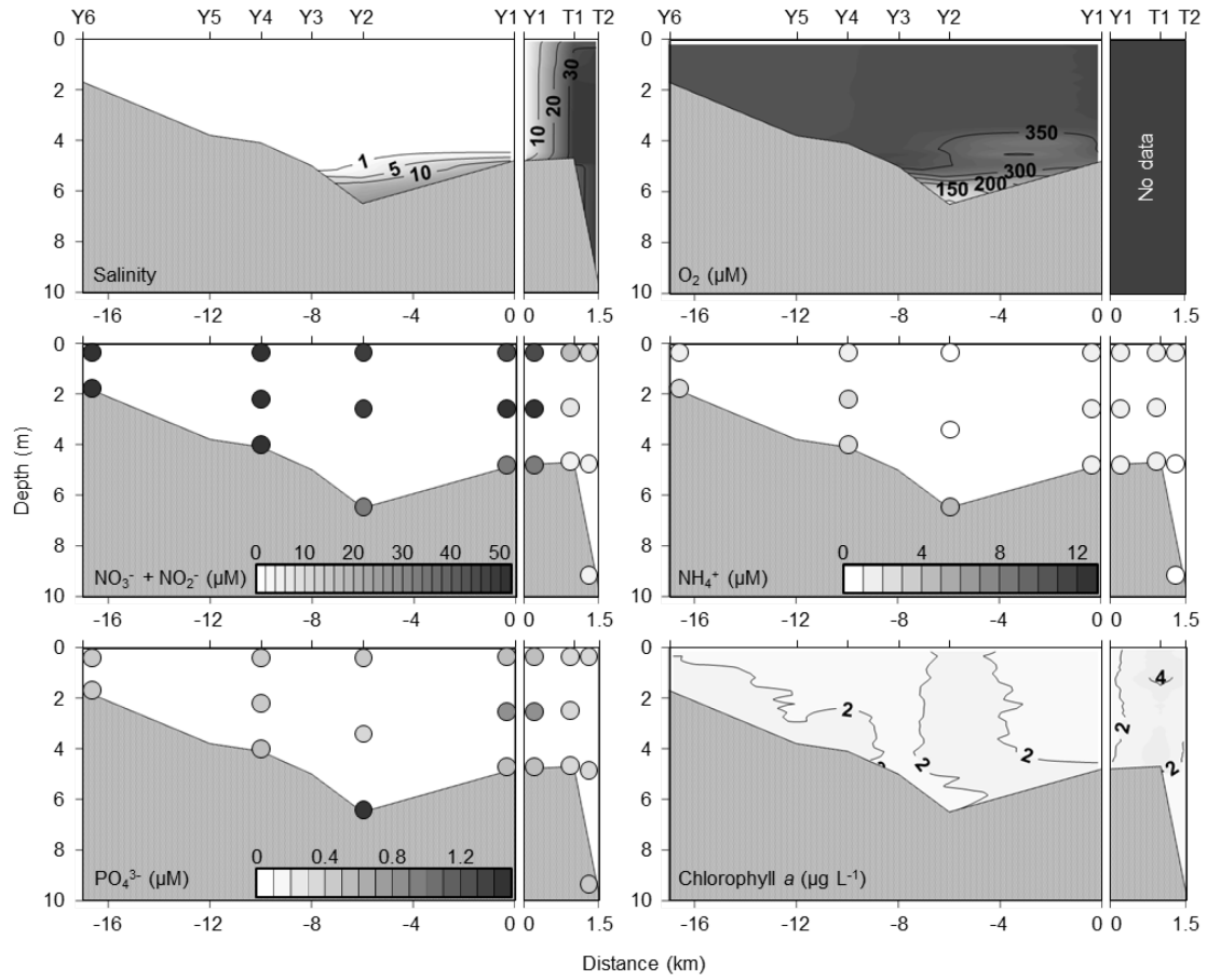
Fig. 2-4. Longitudinal transects of salinity, dissolved oxygen ( \text{O}_2 ), \text{NO}_3^- + \text{NO}_2^- , \text{NH}_4^+ , \text{PO}_4^{3-} , and chlorophyll a along the Yura River estuary on 28–29 January 2008.
