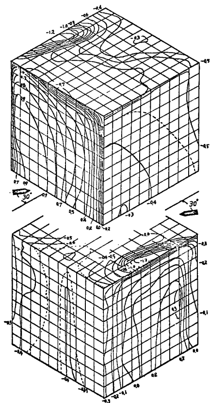
Fig. 5 (c) Distribution of pressure coefficient on a cubic model, angle of attack 30^\circ .
