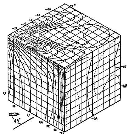
Fig. 5 (d) Distribution of pressure coefficient on a cubic model, angle of attack, 45^\circ .
